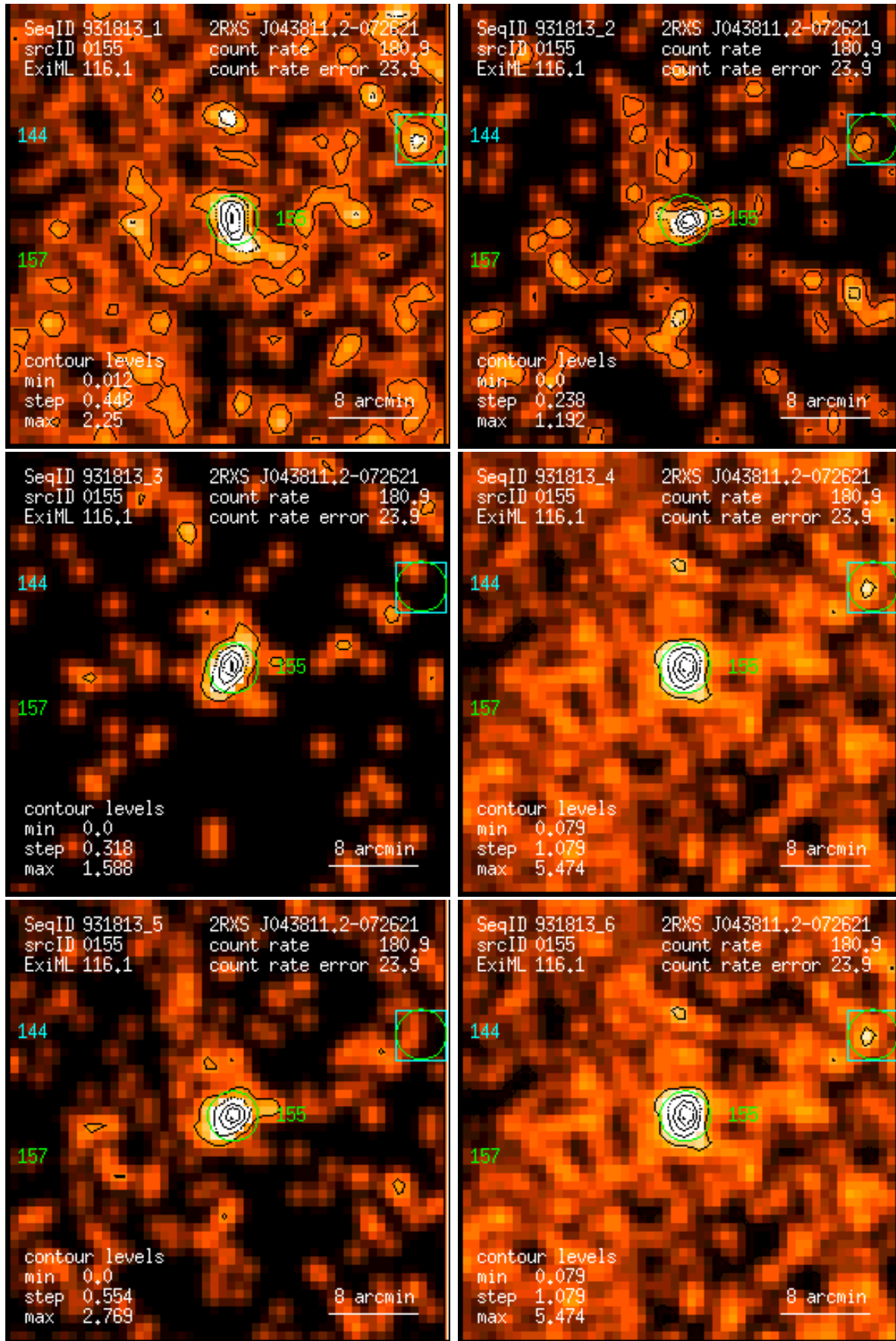
Figure 155: RASS 931813: detection 0155: band rate images, Gaussian filter: (1) PSPC channels 11 – 41, (2) 52 – 90, (3) 91 – 201, (4) 11 – 235, (5) 52 – 201, (6) 11 – 201. Broad band rates in counts/ks. Band rate contour levels in counts/ks/arcmin 2 .
