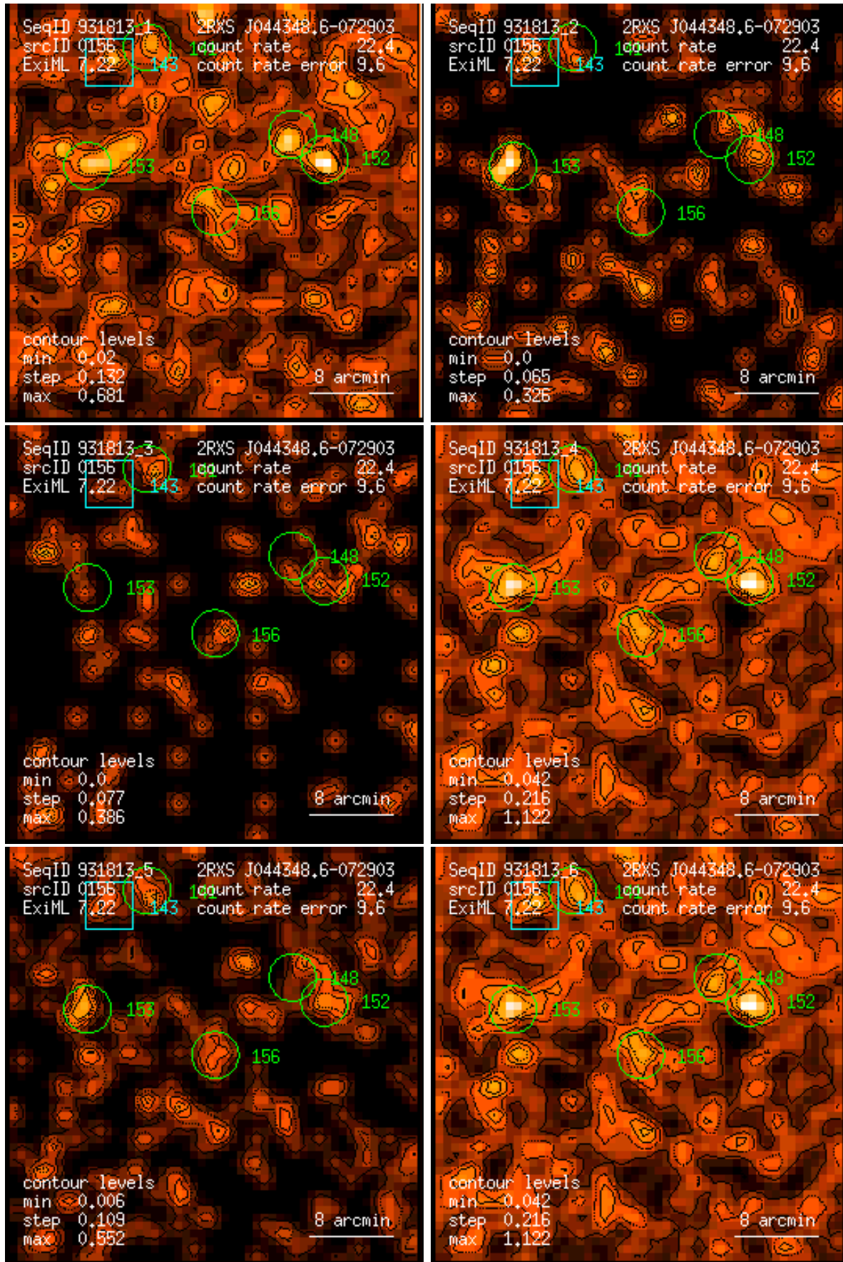
Figure 156: RASS 931813: detection 0156: band rate images, Gaussian filter: (1) PSPC channels 11 – 41, (2) 52 – 90, (3) 91 – 201, (4) 11 – 235, (5) 52 – 201, (6) 11 – 201. Broad band rates in counts/ks. Band rate contour levels in counts/ks/arcmin 2 .
