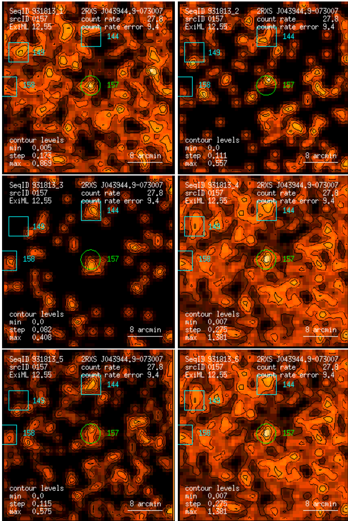
Figure 157: RASS 931813: detection 0157: band rate images, Gaussian filter: (1) PSPC channels 11 – 41, (2) 52 – 90, (3) 91 – 201, (4) 11 – 235, (5) 52 – 201, (6) 11 – 201. Broad band rates in counts/ks. Band rate contour levels in counts/ks/arcmin 2 .
