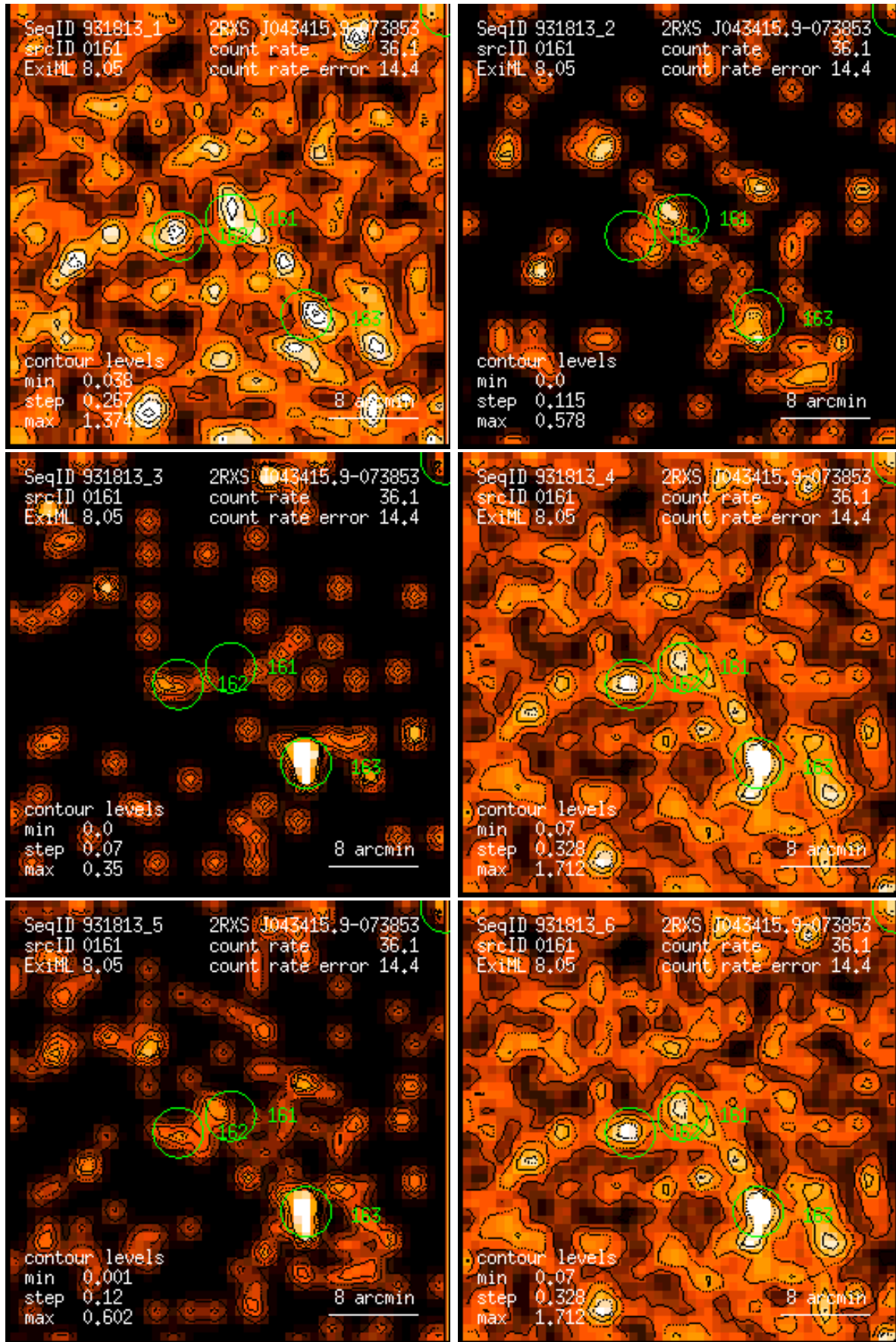
Figure 161: RASS 931813: detection 0161: band rate images, Gaussian filter: (1) PSPC channels 11 – 41, (2) 52 – 90, (3) 91 – 201, (4) 11 – 235, (5) 52 – 201, (6) 11 – 201. Broad band rates in counts/ks. Band rate contour levels in counts/ks/arcmin 2 .
