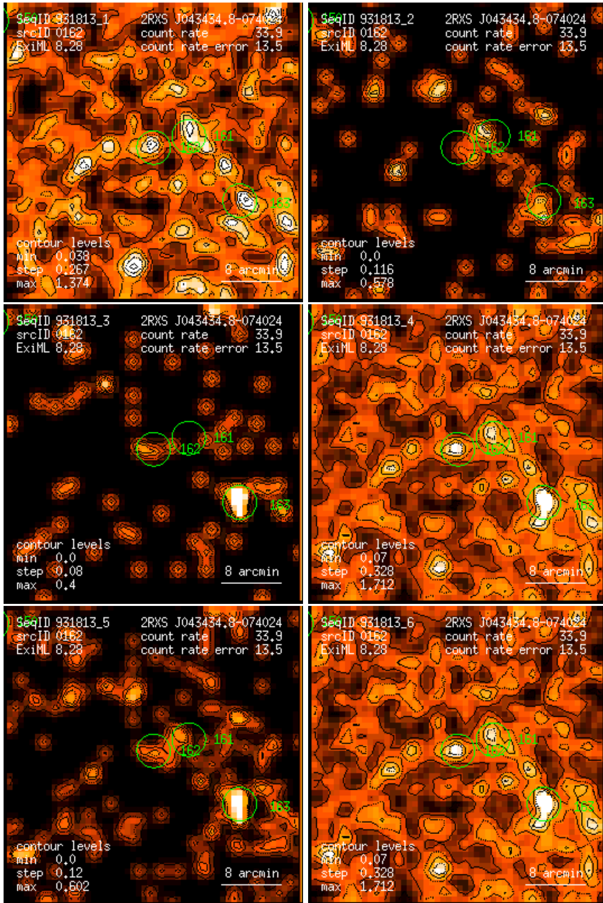
Figure 162: RASS 931813: detection 0162: band rate images, Gaussian filter: (1) PSPC channels 11 – 41, (2) 52 – 90, (3) 91 – 201, (4) 11 – 235, (5) 52 – 201, (6) 11 – 201. Broad band rates in counts/ks. Band rate contour levels in counts/ks/arcmin 2 .
