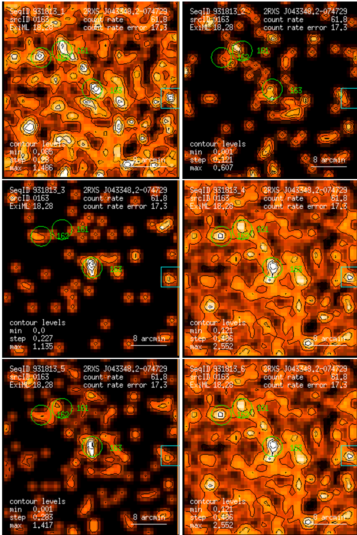
Figure 163: RASS 931813: detection 0163: band rate images, Gaussian filter: (1) PSPC channels 11 – 41, (2) 52 – 90, (3) 91 – 201, (4) 11 – 235, (5) 52 – 201, (6) 11 – 201. Broad band rates in counts/ks. Band rate contour levels in counts/ks/arcmin 2 .
