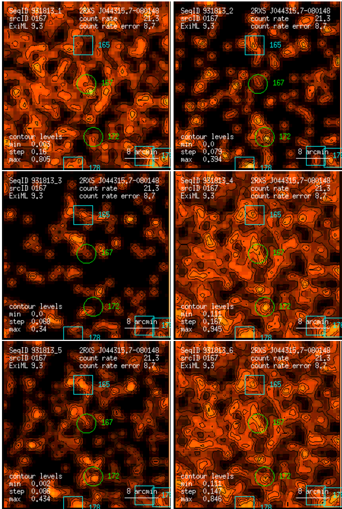
Figure 167: RASS 931813: detection 0167: band rate images, Gaussian filter: (1) PSPC channels 11 – 41, (2) 52 – 90, (3) 91 – 201, (4) 11 – 235, (5) 52 – 201, (6) 11 – 201. Broad band rates in counts/ks. Band rate contour levels in counts/ks/arcmin 2 .
