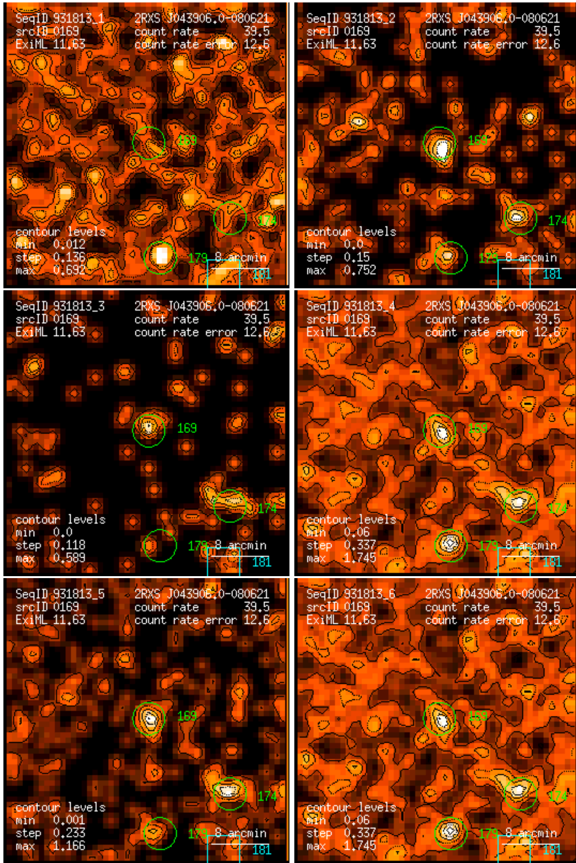
Figure 169: RASS 931813: detection 0169: band rate images, Gaussian filter: (1) PSPC channels 11 – 41, (2) 52 – 90, (3) 91 – 201, (4) 11 – 235, (5) 52 – 201, (6) 11 – 201. Broad band rates in counts/ks. Band rate contour levels in counts/ks/arcmin 2 .
