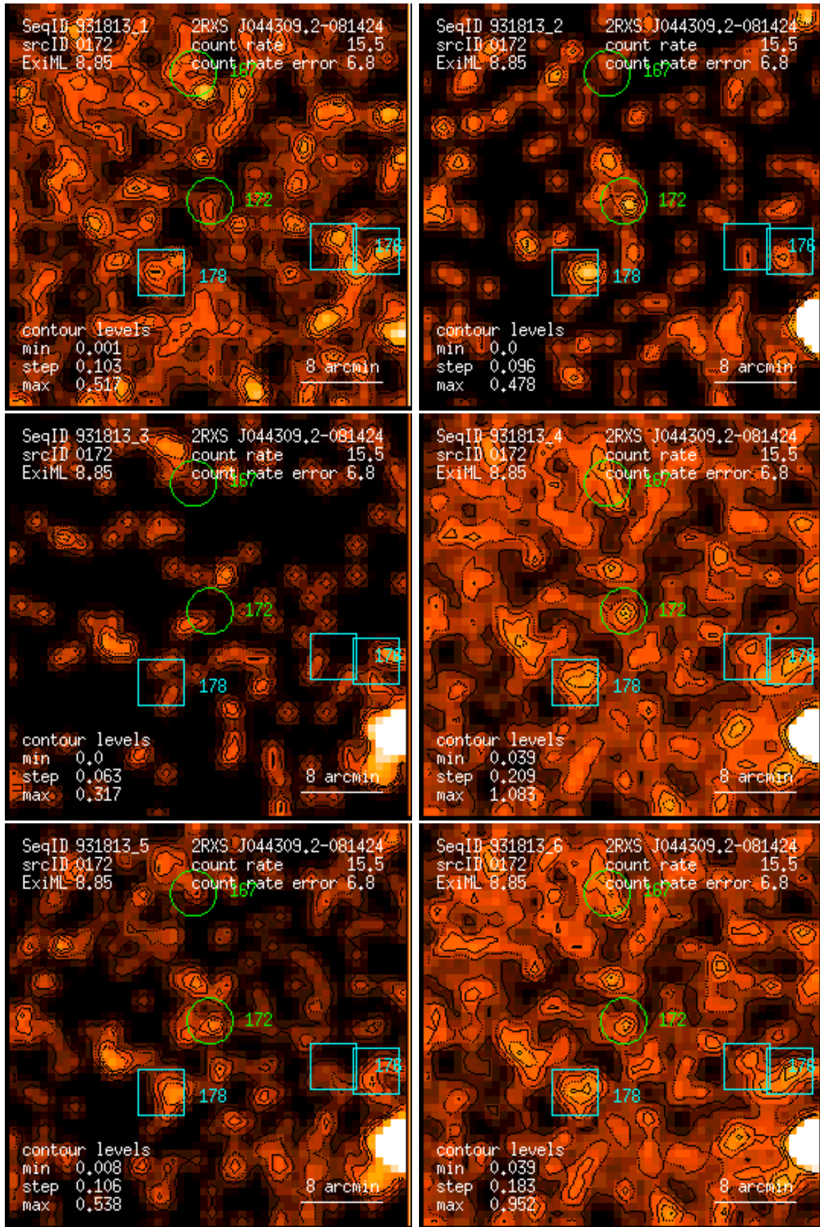
Figure 172: RASS 931813: detection 0172: band rate images, Gaussian filter: (1) PSPC channels 11 – 41, (2) 52 – 90, (3) 91 – 201, (4) 11 – 235, (5) 52 – 201, (6) 11 – 201. Broad band rates in counts/ks. Band rate contour levels in counts/ks/arcmin 2 .
