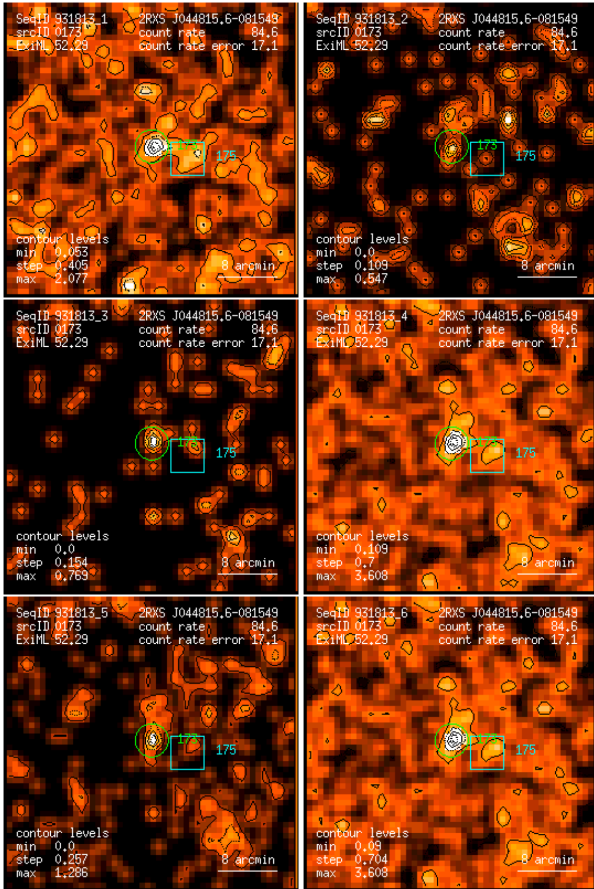
Figure 173: RASS 931813: detection 0173: band rate images, Gaussian filter: (1) PSPC channels 11 – 41, (2) 52 – 90, (3) 91 – 201, (4) 11 – 235, (5) 52 – 201, (6) 11 – 201. Broad band rates in counts/ks. Band rate contour levels in counts/ks/arcmin 2 .
