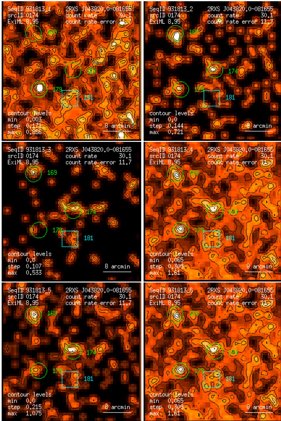
Figure 174: RASS 931813: detection 0174: band rate images, Gaussian filter: (1) PSPC channels 11 – 41, (2) 52 – 90, (3) 91 – 201, (4) 11 – 235, (5) 52 – 201, (6) 11 – 201. Broad band rates in counts/ks. Band rate contour levels in counts/ks/arcmin 2 .
