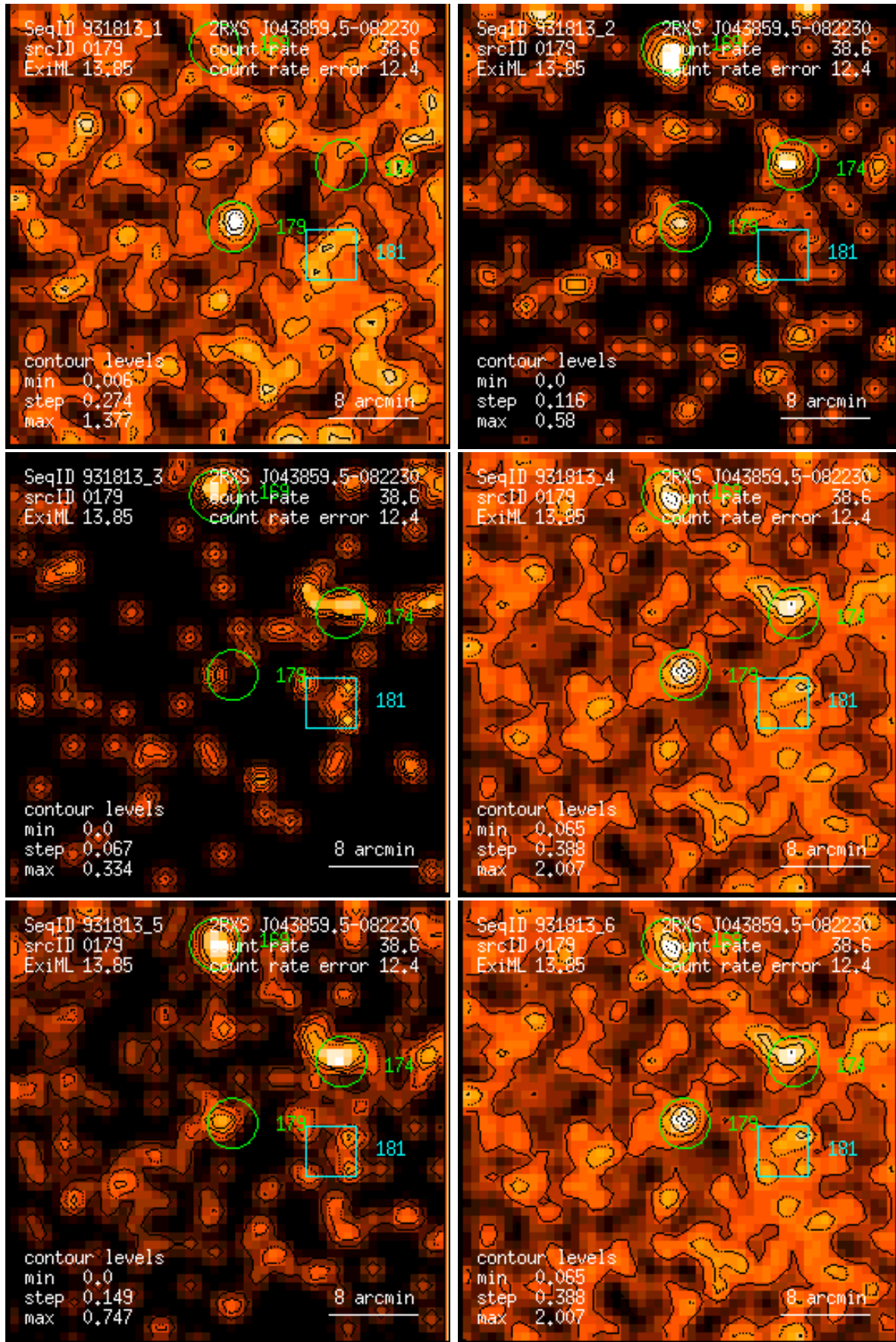
Figure 179: RASS 931813: detection 0179: band rate images, Gaussian filter: (1) PSPC channels 11 – 41, (2) 52 – 90, (3) 91 – 201, (4) 11 – 235, (5) 52 – 201, (6) 11 – 201. Broad band rates in counts/ks. Band rate contour levels in counts/ks/arcmin 2 .
