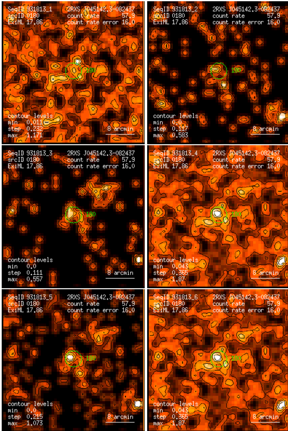
Figure 180: RASS 931813: detection 0180: band rate images, Gaussian filter: (1) PSPC channels 11 – 41, (2) 52 – 90, (3) 91 – 201, (4) 11 – 235, (5) 52 – 201, (6) 11 – 201. Broad band rates in counts/ks. Band rate contour levels in counts/ks/arcmin 2 .
