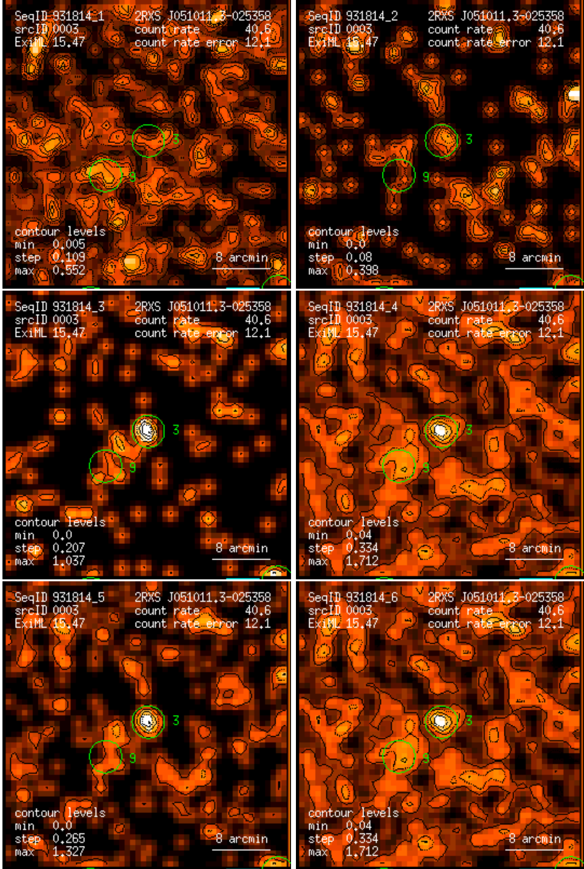
Figure 3: RASS 931814: detection 0003: band rate images, Gaussian filter: (1) PSPC channels 11 – 41, (2) 52 – 90, (3) 91 – 201, (4) 11 – 235, (5) 52 – 201, (6) 11 – 201. Broad band rates in counts/ks. Band rate contour levels in counts/ks/arcmin 2 .
