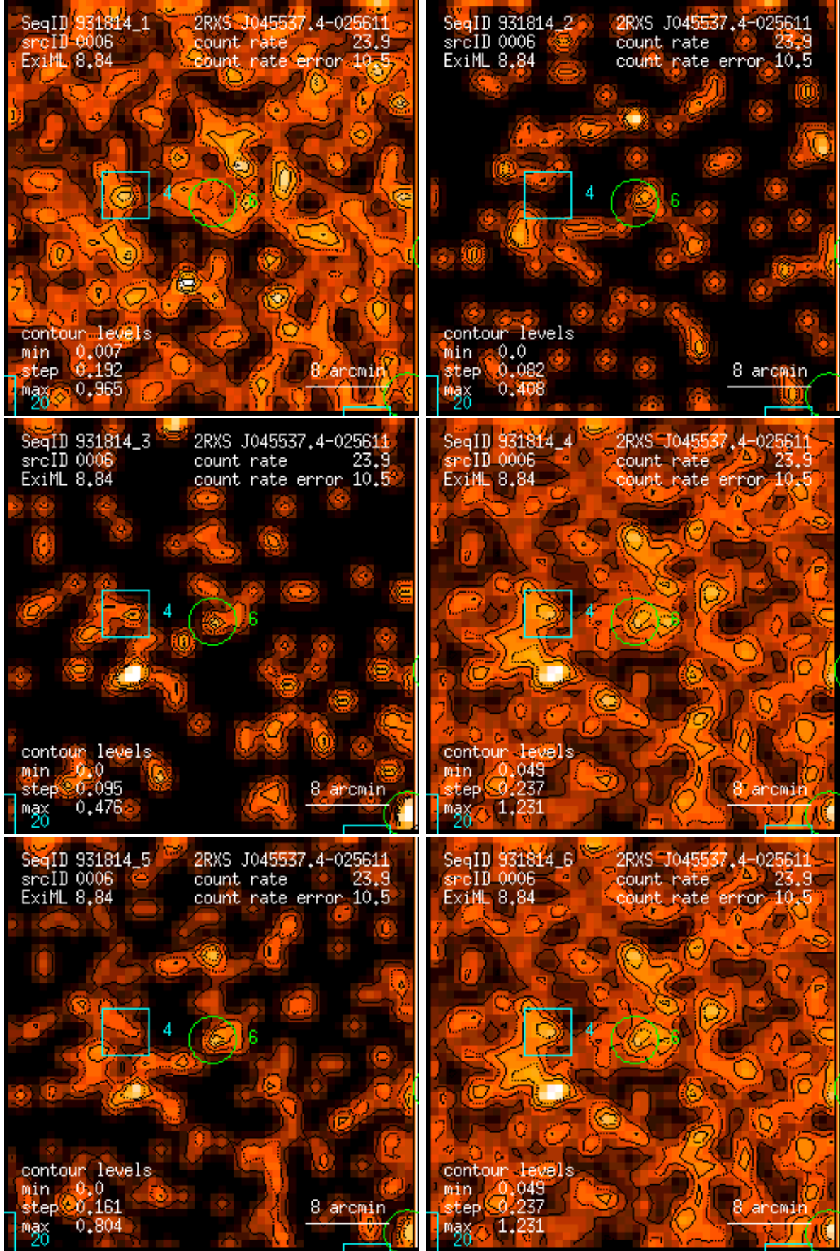
Figure 6: RASS 931814: detection 0006: band rate images, Gaussian filter: (1) PSPC channels 11 – 41, (2) 52 – 90, (3) 91 – 201, (4) 11 – 235, (5) 52 – 201, (6) 11 – 201. Broad band rates in counts/ks. Band rate contour levels in counts/ks/arcmin 2 .
