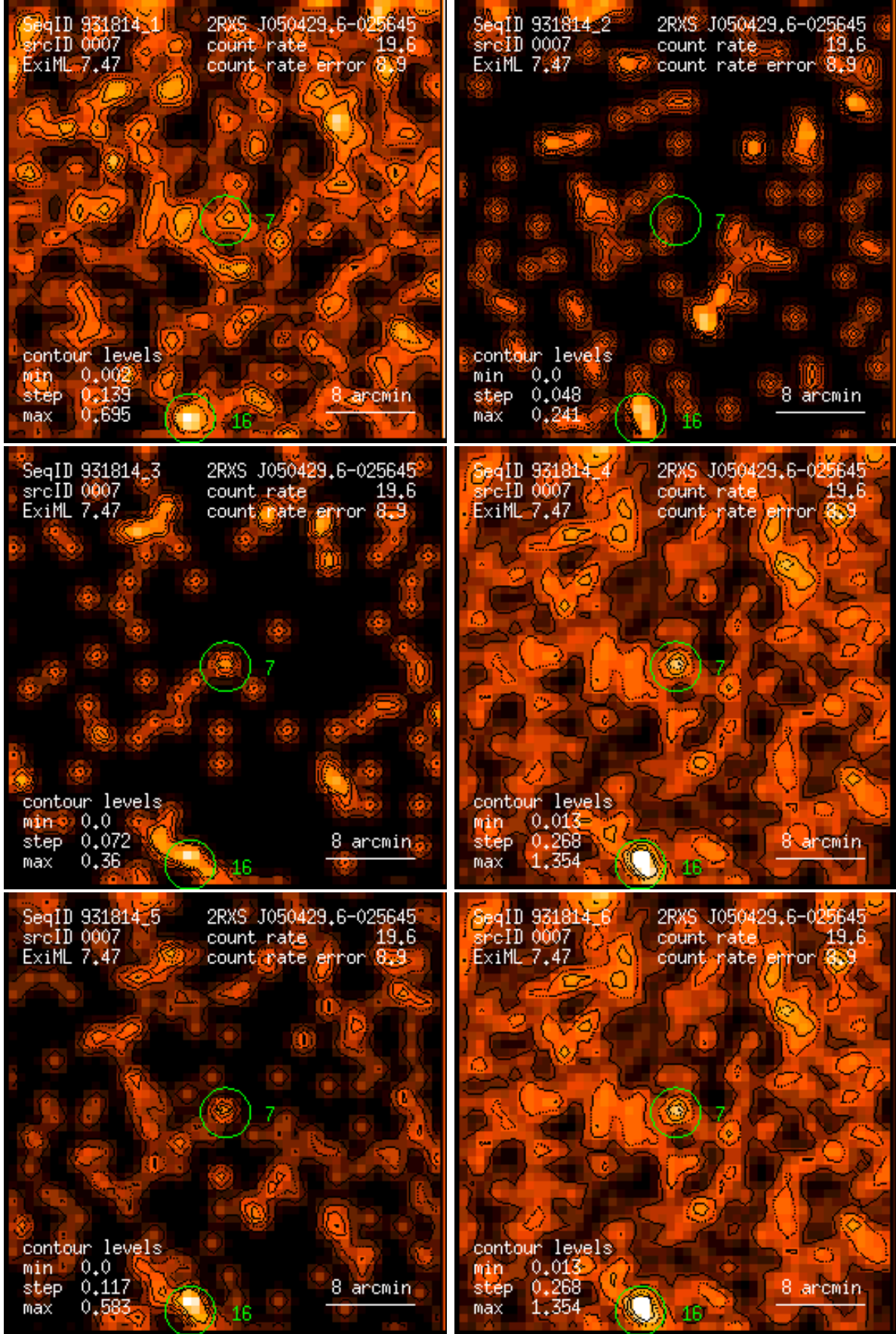
Figure 7: RASS 931814: detection 0007: band rate images, Gaussian filter: (1) PSPC channels 11 – 41, (2) 52 – 90, (3) 91 – 201, (4) 11 – 235, (5) 52 – 201, (6) 11 – 201. Broad band rates in counts/ks. Band rate contour levels in counts/ks/arcmin 2 .
