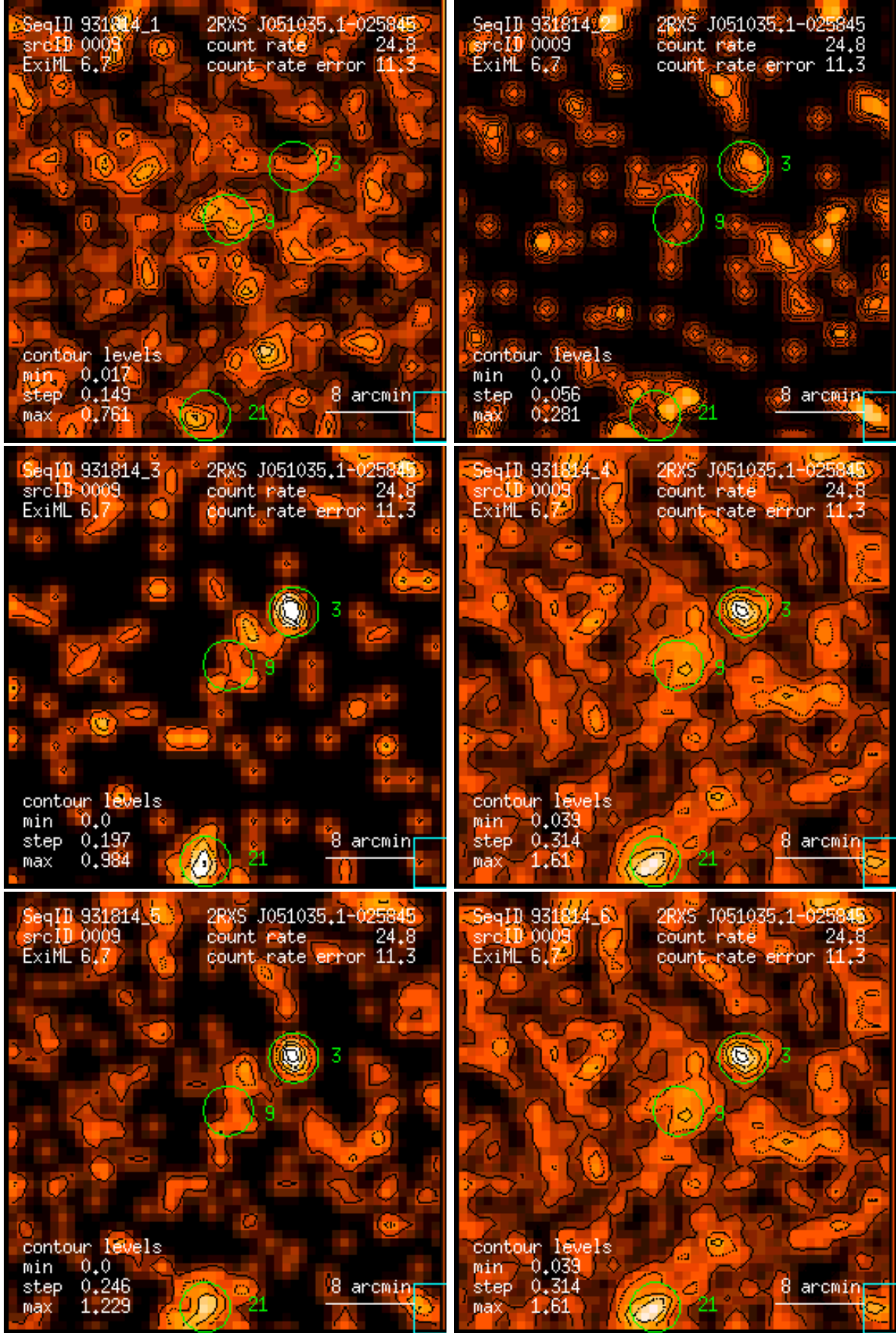
Figure 9: RASS 931814: detection 0009: band rate images, Gaussian filter: (1) PSPC channels 11 – 41, (2) 52 – 90, (3) 91 – 201, (4) 11 – 235, (5) 52 – 201, (6) 11 – 201. Broad band rates in counts/ks. Band rate contour levels in counts/ks/arcmin 2 .
