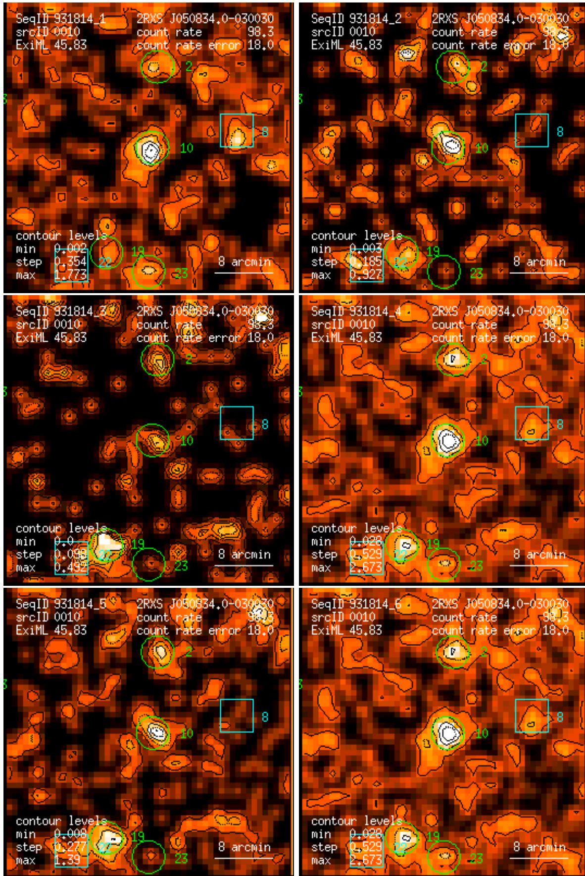
Figure 10: RASS 931814: detection 0010: band rate images, Gaussian filter: (1) PSPC channels 11 – 41, (2) 52 – 90, (3) 91 – 201, (4) 11 – 235, (5) 52 – 201, (6) 11 – 201. Broad band rates in counts/ks. Band rate contour levels in counts/ks/arcmin 2 .
