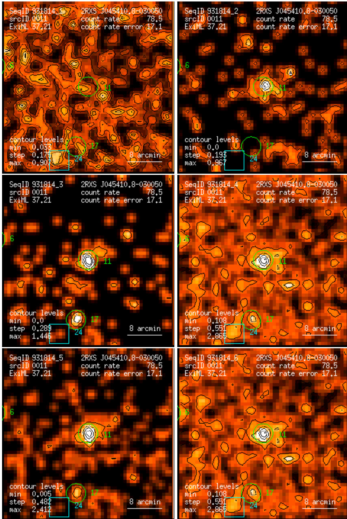
Figure 11: RASS 931814: detection 0011: band rate images, Gaussian filter: (1) PSPC channels 11 – 41, (2) 52 – 90, (3) 91 – 201, (4) 11 – 235, (5) 52 – 201, (6) 11 – 201. Broad band rates in counts/ks. Band rate contour levels in counts/ks/arcmin 2 .
