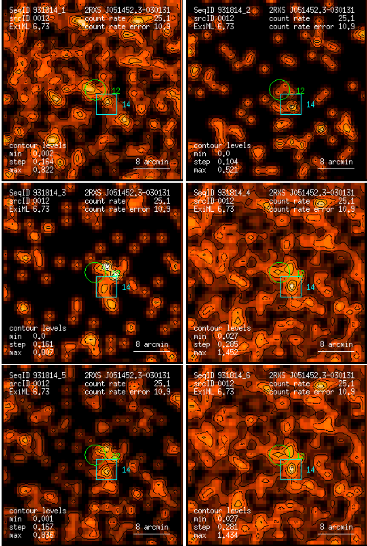
Figure 12: RASS 931814: detection 0012: band rate images, Gaussian filter: (1) PSPC channels 11 – 41, (2) 52 – 90, (3) 91 – 201, (4) 11 – 235, (5) 52 – 201, (6) 11 – 201. Broad band rates in counts/ks. Band rate contour levels in counts/ks/arcmin 2 .
