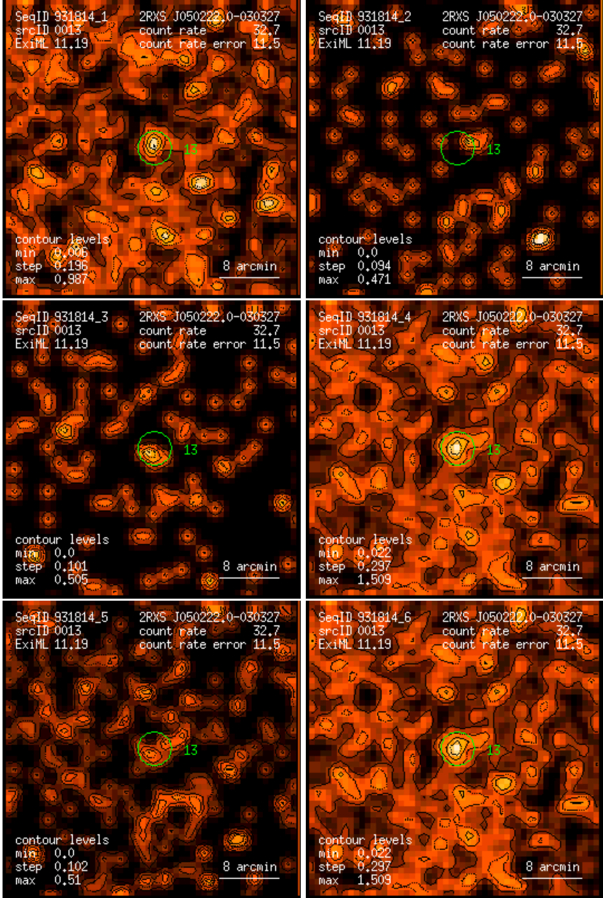
Figure 13: RASS 931814: detection 0013: band rate images, Gaussian filter: (1) PSPC channels 11 – 41, (2) 52 – 90, (3) 91 – 201, (4) 11 – 235, (5) 52 – 201, (6) 11 – 201. Broad band rates in counts/ks. Band rate contour levels in counts/ks/arcmin 2 .
