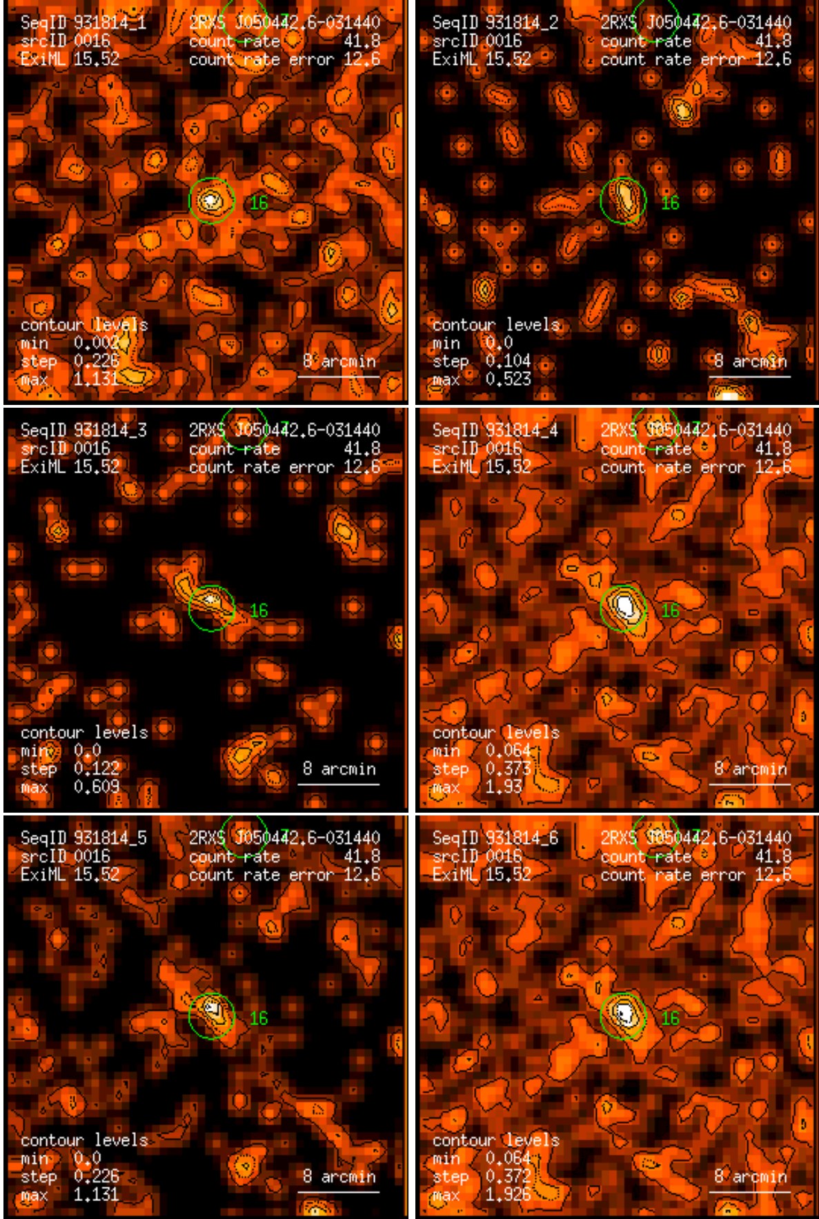
Figure 16: RASS 931814: detection 0016: band rate images, Gaussian filter: (1) PSPC channels 11 – 41, (2) 52 – 90, (3) 91 – 201, (4) 11 – 235, (5) 52 – 201, (6) 11 – 201. Broad band rates in counts/ks. Band rate contour levels in counts/ks/arcmin 2 .
