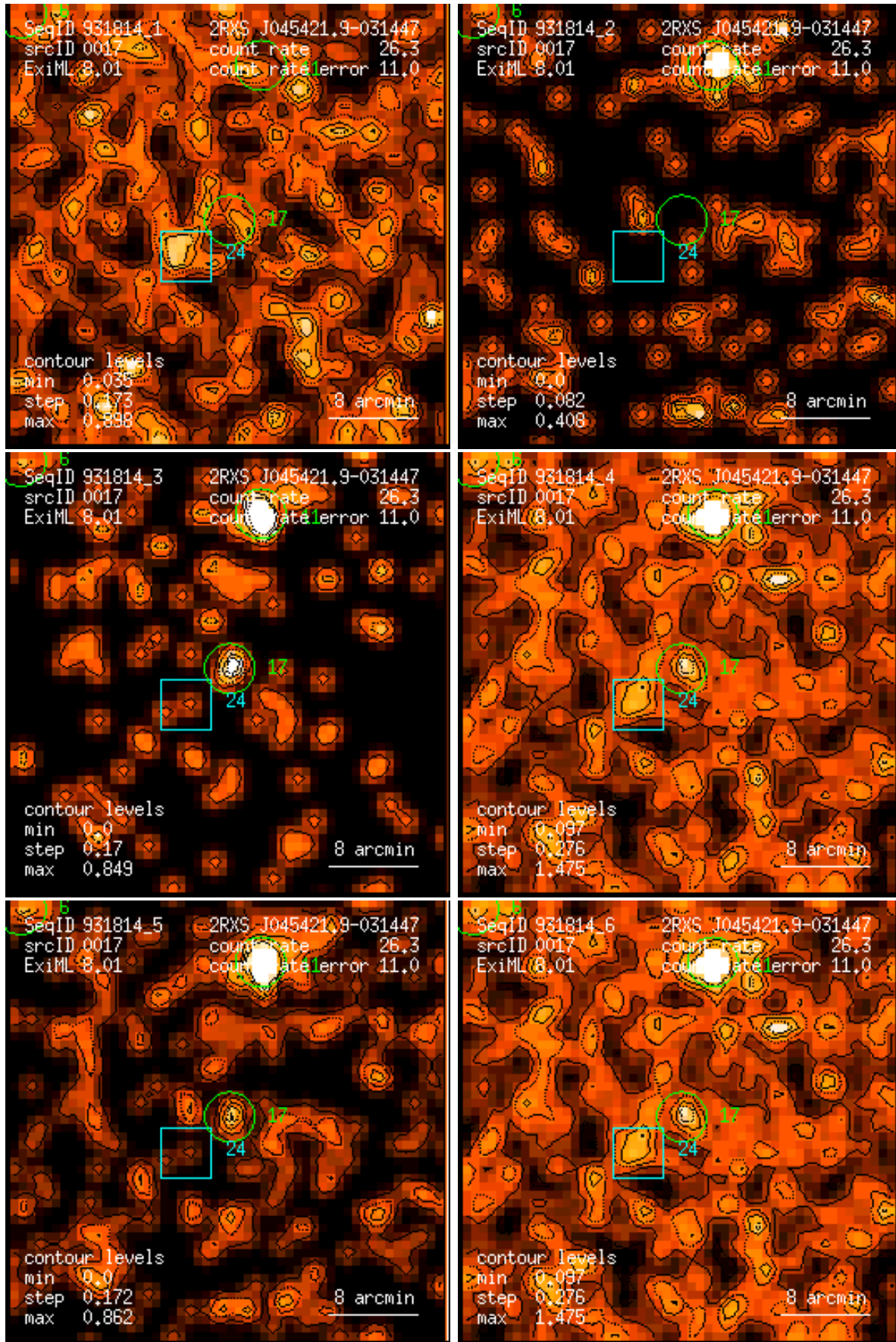
Figure 17: RASS 931814: detection 0017: band rate images, Gaussian filter: (1) PSPC channels 11 – 41, (2) 52 – 90, (3) 91 – 201, (4) 11 – 235, (5) 52 – 201, (6) 11 – 201. Broad band rates in counts/ks. Band rate contour levels in counts/ks/arcmin 2 .
