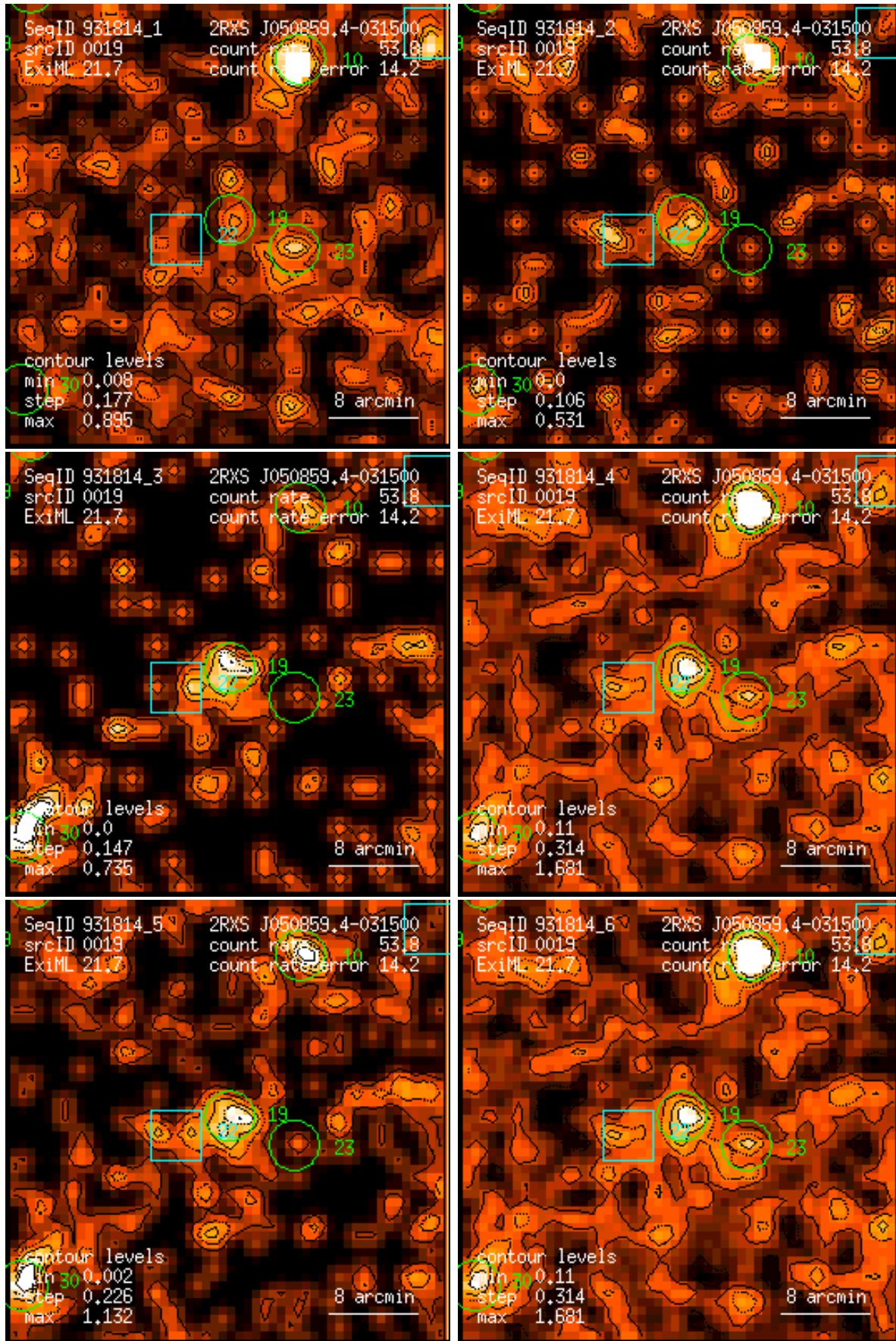
Figure 19: RASS 931814: detection 0019: band rate images, Gaussian filter: (1) PSPC channels 11 – 41, (2) 52 – 90, (3) 91 – 201, (4) 11 – 235, (5) 52 – 201, (6) 11 – 201. Broad band rates in counts/ks. Band rate contour levels in counts/ks/arcmin 2 .
