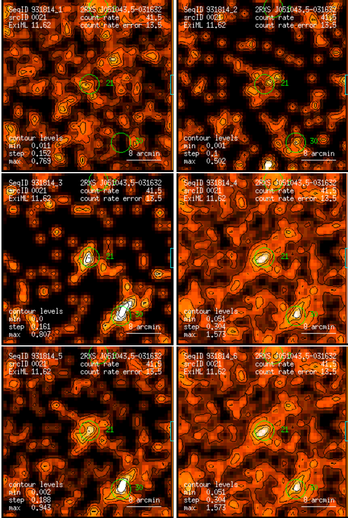
Figure 21: RASS 931814: detection 0021: band rate images, Gaussian filter: (1) PSPC channels 11 – 41, (2) 52 – 90, (3) 91 – 201, (4) 11 – 235, (5) 52 – 201, (6) 11 – 201. Broad band rates in counts/ks. Band rate contour levels in counts/ks/arcmin 2 .
