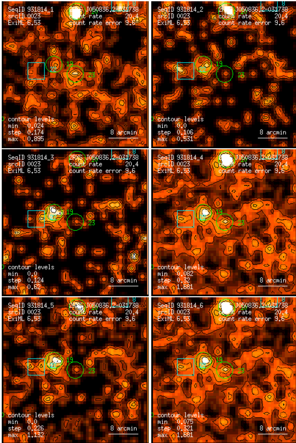
Figure 23: RASS 931814: detection 0023: band rate images, Gaussian filter: (1) PSPC channels 11 – 41, (2) 52 – 90, (3) 91 – 201, (4) 11 – 235, (5) 52 – 201, (6) 11 – 201. Broad band rates in counts/ks. Band rate contour levels in counts/ks/arcmin 2 .
