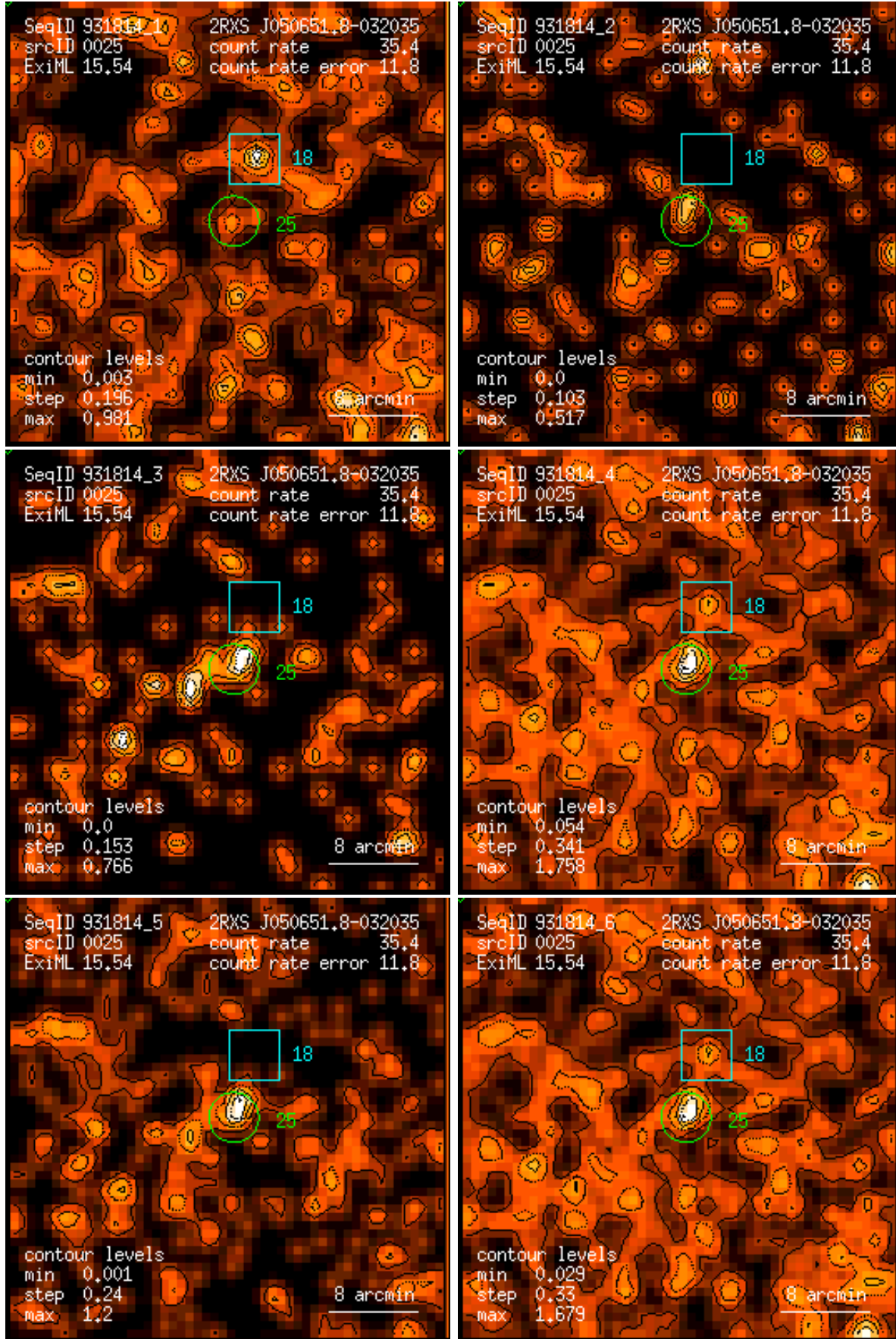
Figure 25: RASS 931814: detection 0025: band rate images, Gaussian filter: (1) PSPC channels 11 – 41, (2) 52 – 90, (3) 91 – 201, (4) 11 – 235, (5) 52 – 201, (6) 11 – 201. Broad band rates in counts/ks. Band rate contour levels in counts/ks/arcmin 2 .
