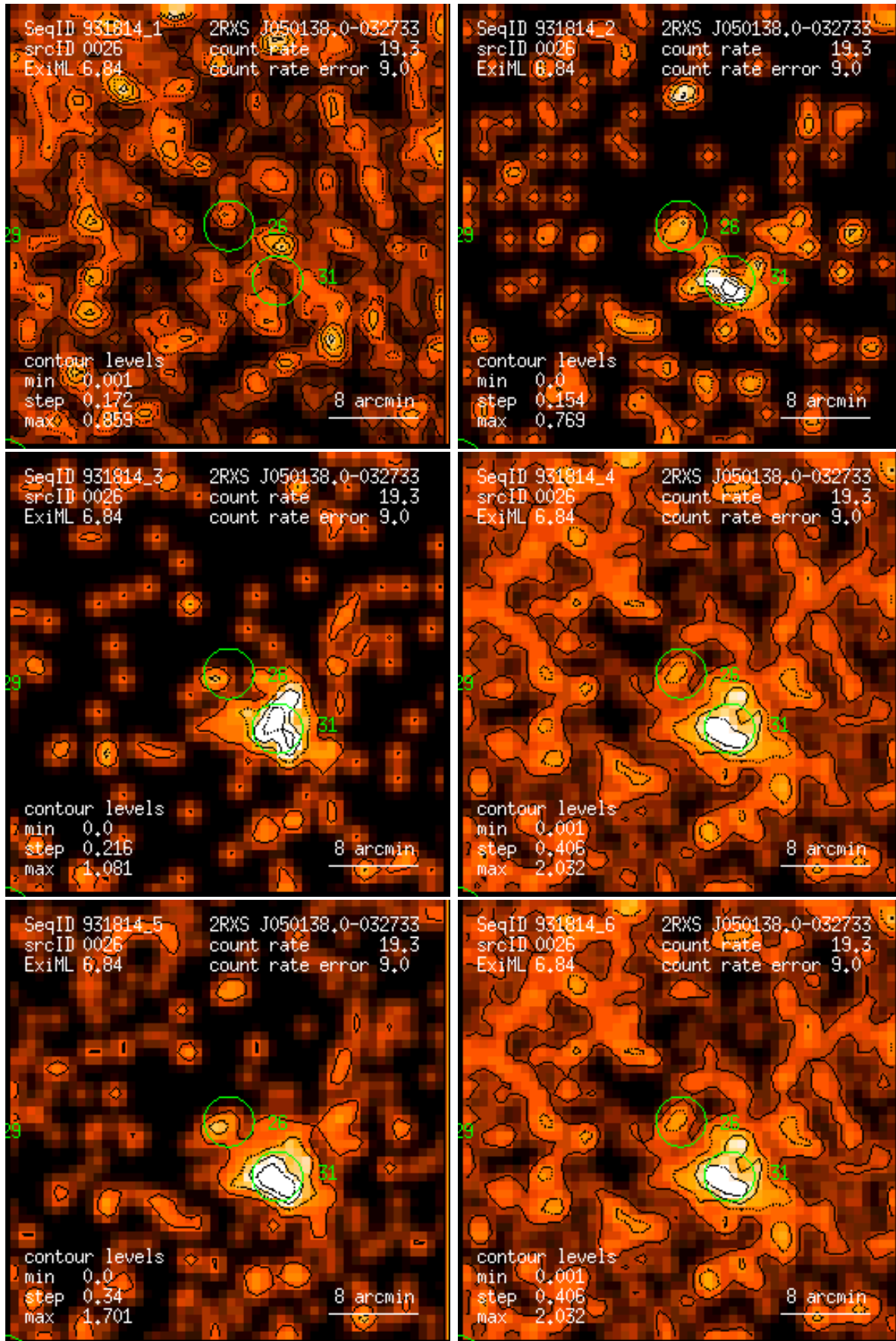
Figure 26: RASS 931814: detection 0026: band rate images, Gaussian filter: (1) PSPC channels 11 – 41, (2) 52 – 90, (3) 91 – 201, (4) 11 – 235, (5) 52 – 201, (6) 11 – 201. Broad band rates in counts/ks. Band rate contour levels in counts/ks/arcmin 2 .
