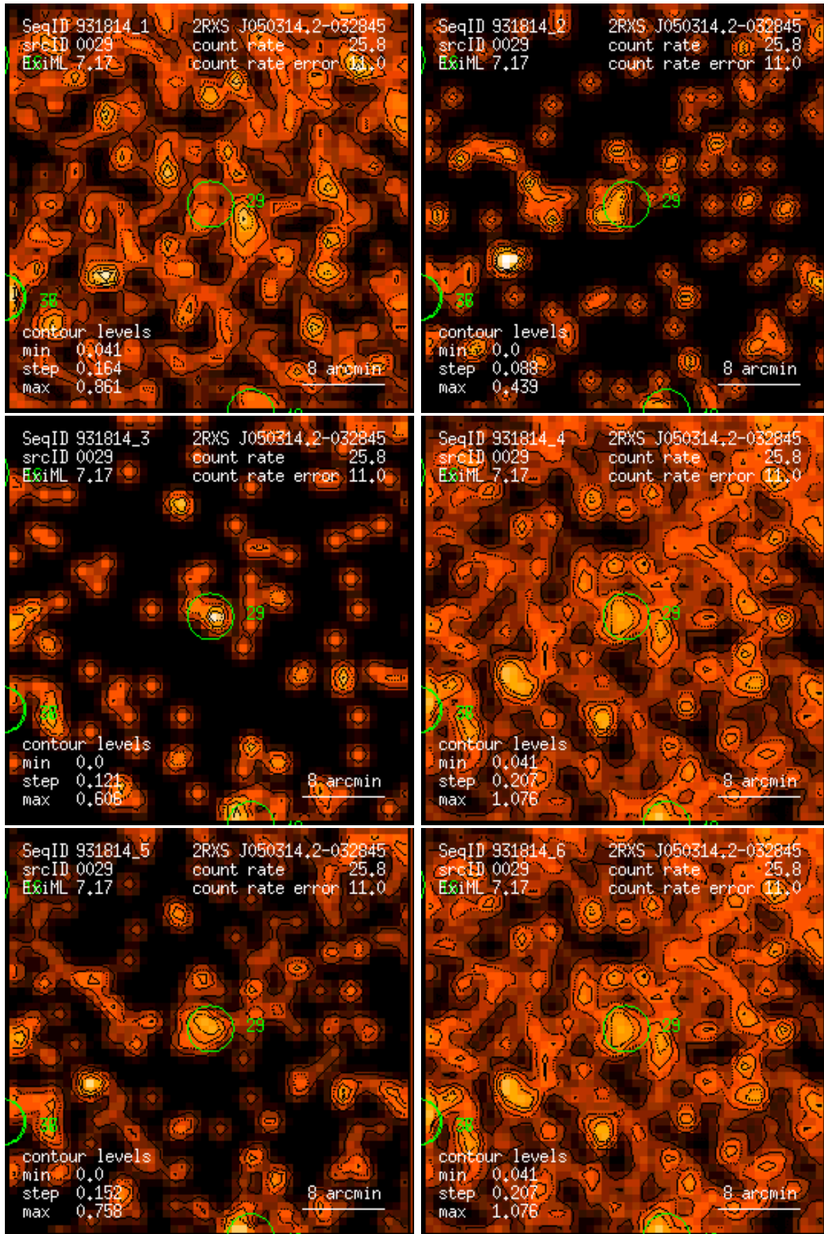
Figure 29: RASS 931814: detection 0029: band rate images, Gaussian filter: (1) PSPC channels 11 – 41, (2) 52 – 90, (3) 91 – 201, (4) 11 – 235, (5) 52 – 201, (6) 11 – 201. Broad band rates in counts/ks. Band rate contour levels in counts/ks/arcmin 2 .
