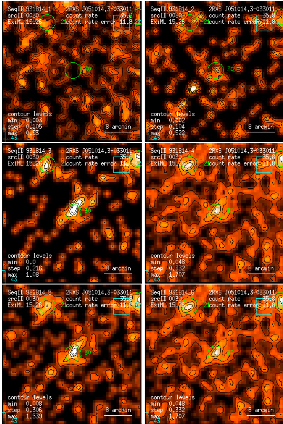
Figure 30: RASS 931814: detection 0030: band rate images, Gaussian filter: (1) PSPC channels 11 – 41, (2) 52 – 90, (3) 91 – 201, (4) 11 – 235, (5) 52 – 201, (6) 11 – 201. Broad band rates in counts/ks. Band rate contour levels in counts/ks/arcmin 2 .
