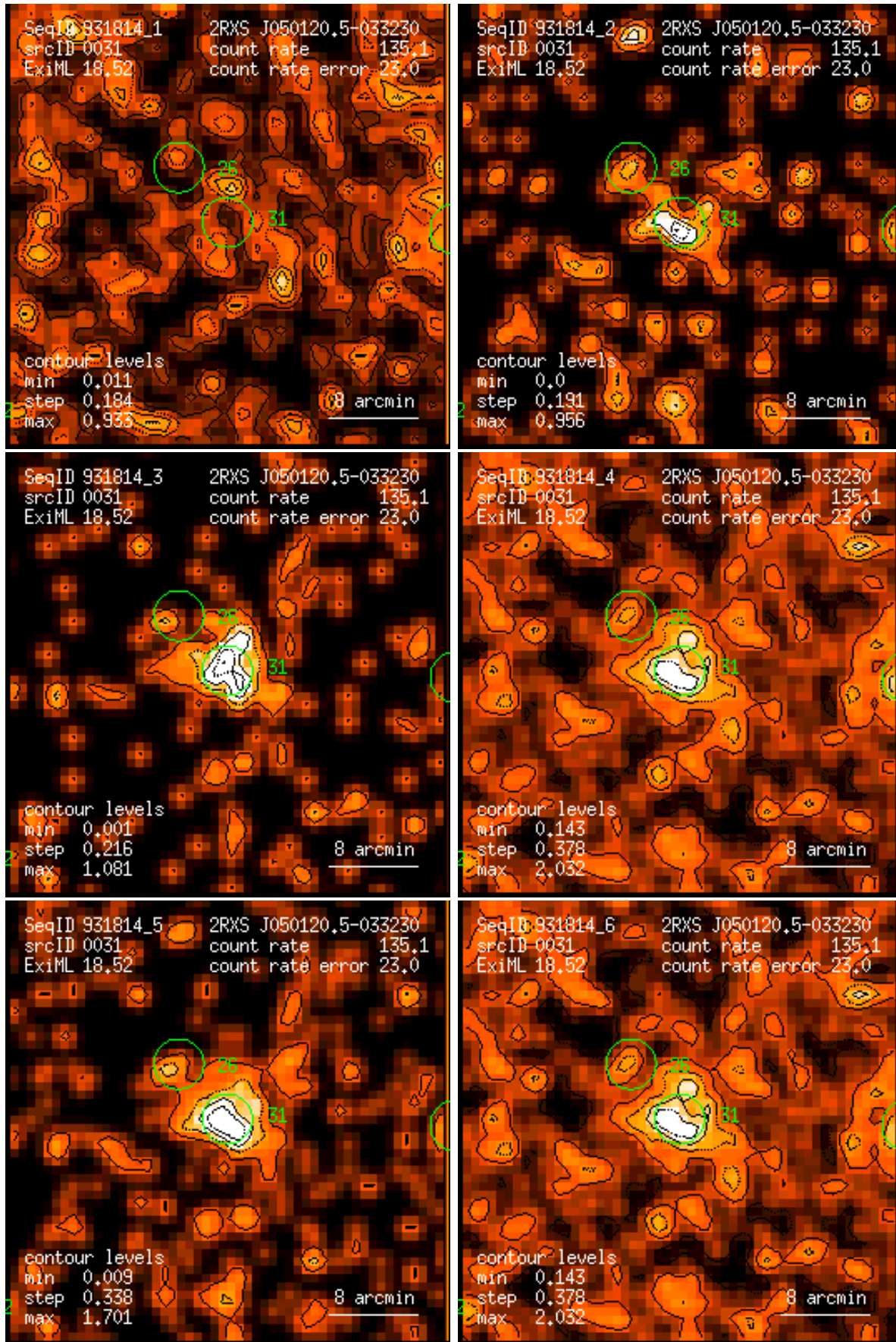
Figure 31: RASS 931814: detection 0031: band rate images, Gaussian filter: (1) PSPC channels 11 – 41, (2) 52 – 90, (3) 91 – 201, (4) 11 – 235, (5) 52 – 201, (6) 11 – 201. Broad band rates in counts/ks. Band rate contour levels in counts/ks/arcmin 2 .
