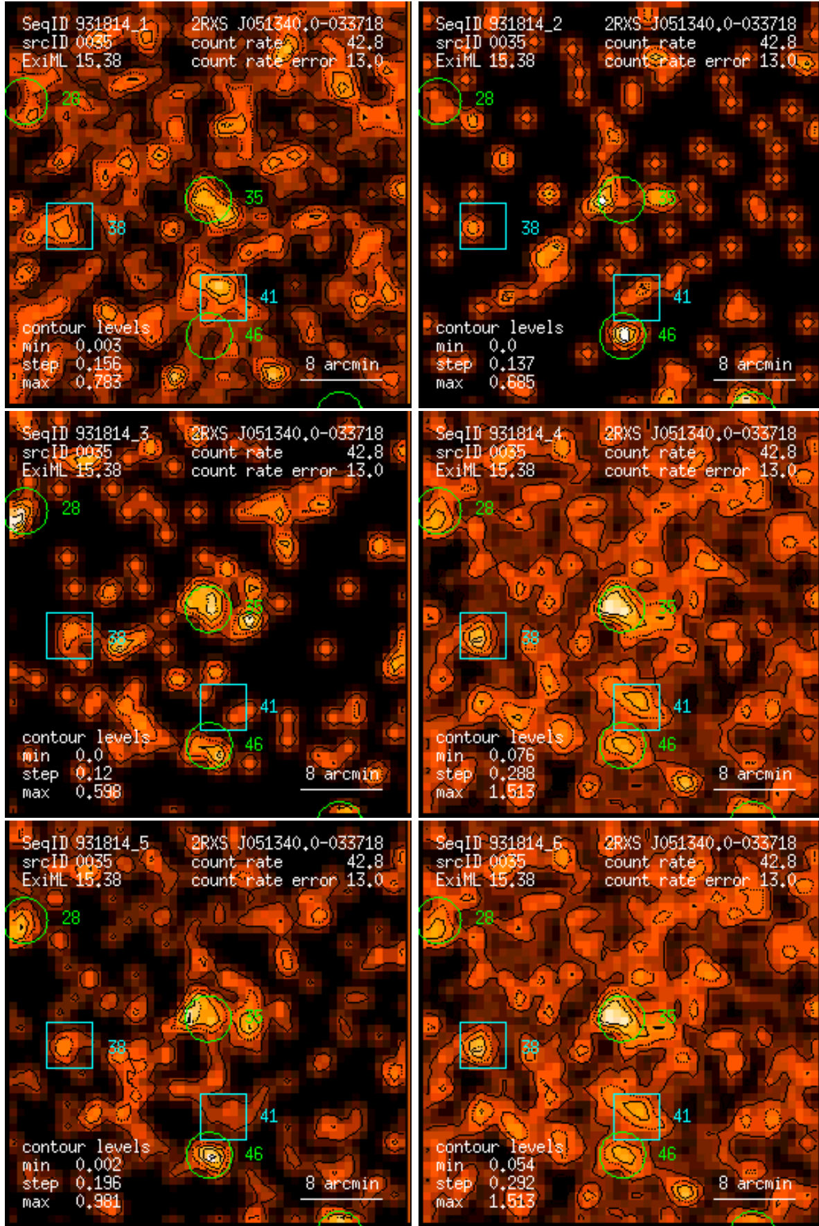
Figure 35: RASS 931814: detection 0035: band rate images, Gaussian filter: (1) PSPC channels 11 – 41, (2) 52 – 90, (3) 91 – 201, (4) 11 – 235, (5) 52 – 201, (6) 11 – 201. Broad band rates in counts/ks. Band rate contour levels in counts/ks/arcmin 2 .
