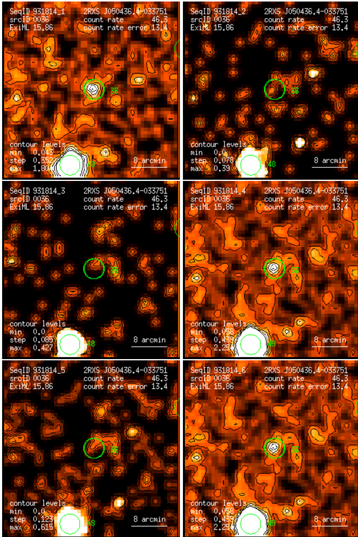
Figure 36: RASS 931814: detection 0036: band rate images, Gaussian filter: (1) PSPC channels 11 – 41, (2) 52 – 90, (3) 91 – 201, (4) 11 – 235, (5) 52 – 201, (6) 11 – 201. Broad band rates in counts/ks. Band rate contour levels in counts/ks/arcmin 2 .
