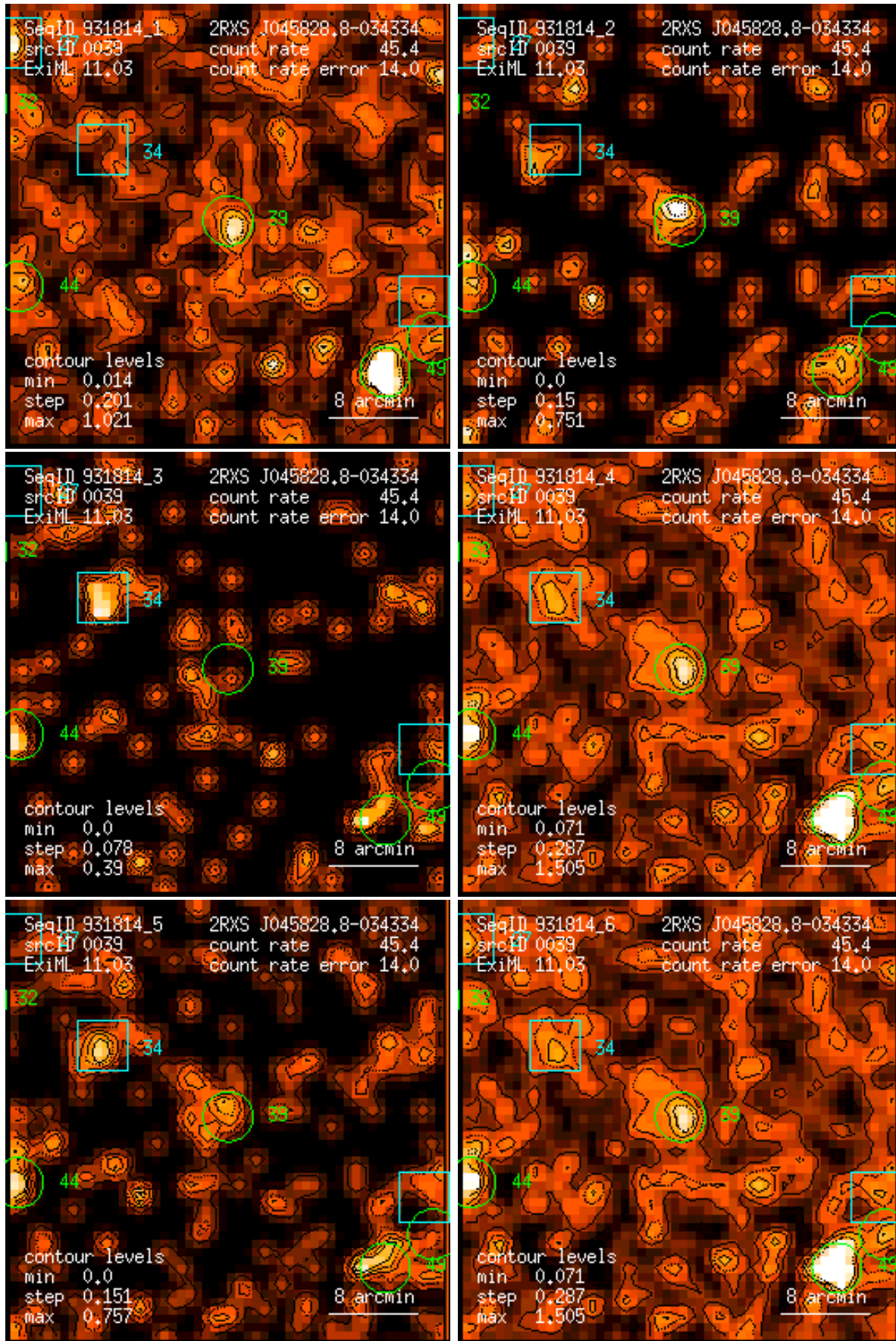
Figure 39: RASS 931814: detection 0039: band rate images, Gaussian filter: (1) PSPC channels 11 – 41, (2) 52 – 90, (3) 91 – 201, (4) 11 – 235, (5) 52 – 201, (6) 11 – 201. Broad band rates in counts/ks. Band rate contour levels in counts/ks/arcmin 2 .
