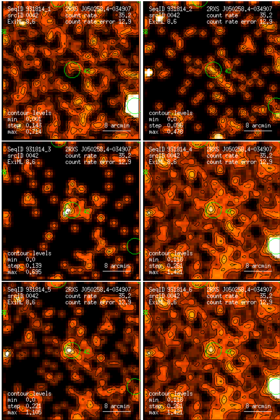
Figure 42: RASS 931814: detection 0042: band rate images, Gaussian filter: (1) PSPC channels 11 – 41, (2) 52 – 90, (3) 91 – 201, (4) 11 – 235, (5) 52 – 201, (6) 11 – 201. Broad band rates in counts/ks. Band rate contour levels in counts/ks/arcmin 2 .
