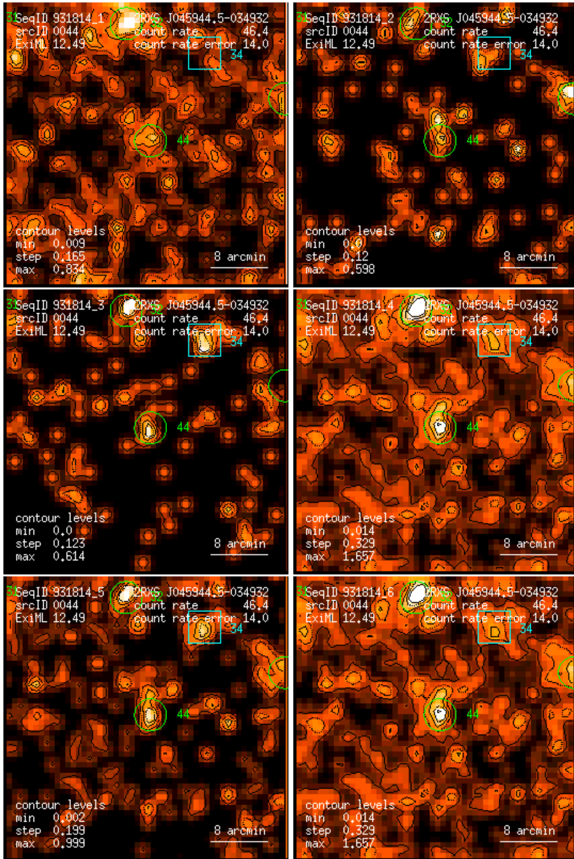
Figure 44: RASS 931814: detection 0044: band rate images, Gaussian filter: (1) PSPC channels 11 – 41, (2) 52 – 90, (3) 91 – 201, (4) 11 – 235, (5) 52 – 201, (6) 11 – 201. Broad band rates in counts/ks. Band rate contour levels in counts/ks/arcmin 2 .
