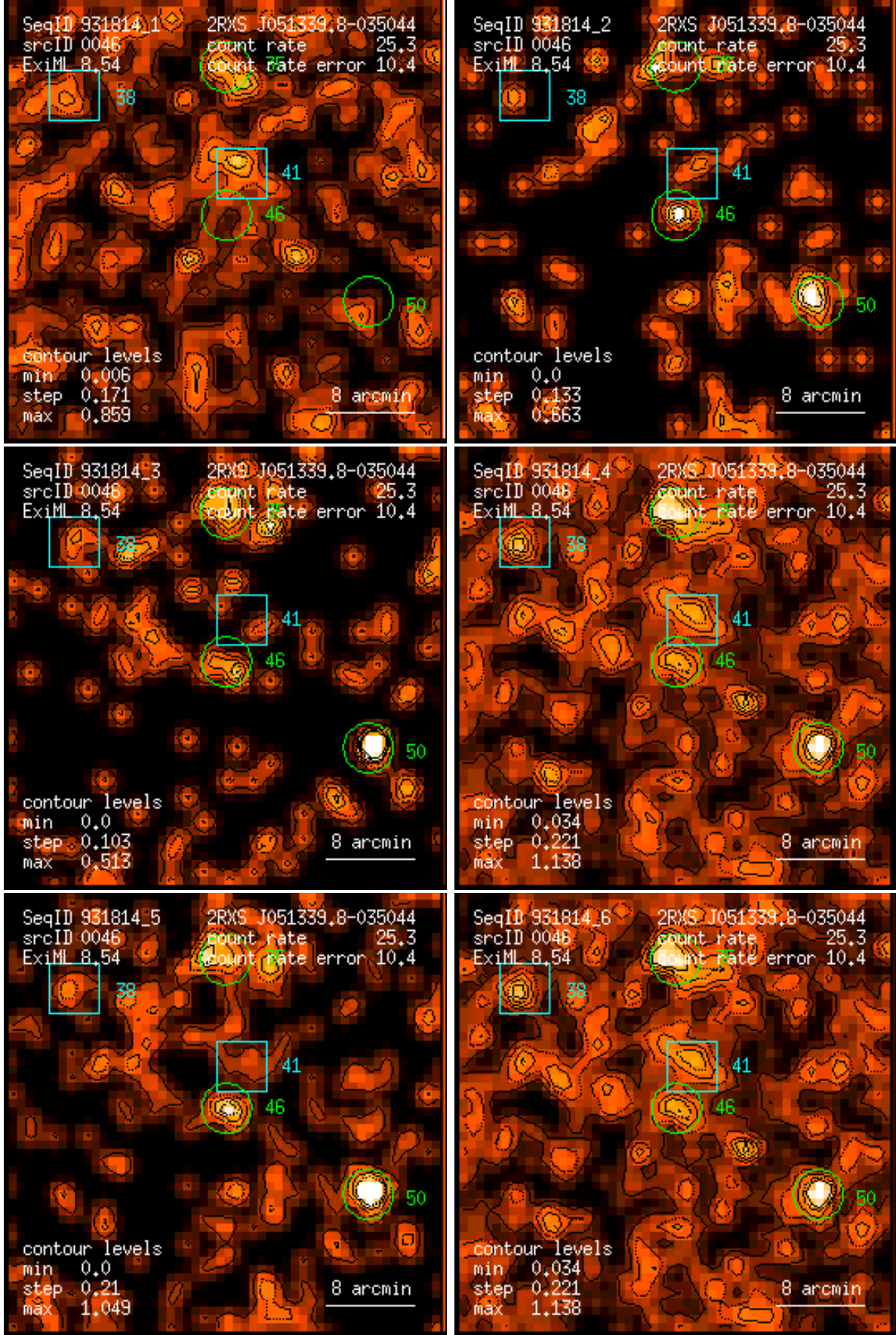
Figure 46: RASS 931814: detection 0046: band rate images, Gaussian filter: (1) PSPC channels 11 – 41, (2) 52 – 90, (3) 91 – 201, (4) 11 – 235, (5) 52 – 201, (6) 11 – 201. Broad band rates in counts/ks. Band rate contour levels in counts/ks/arcmin 2 .
