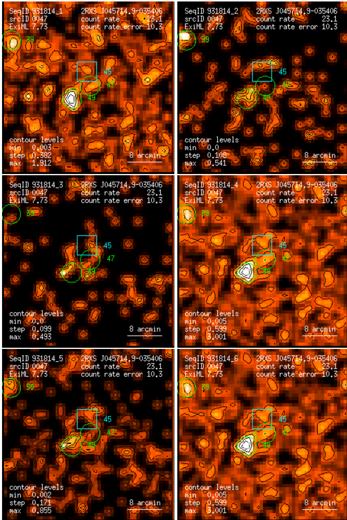
Figure 47: RASS 931814: detection 0047: band rate images, Gaussian filter: (1) PSPC channels 11 – 41, (2) 52 – 90, (3) 91 – 201, (4) 11 – 235, (5) 52 – 201, (6) 11 – 201. Broad band rates in counts/ks. Band rate contour levels in counts/ks/arcmin 2 .
