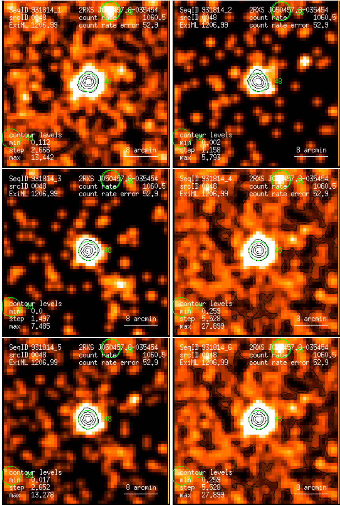
Figure 48: RASS 931814: detection 0048: band rate images, Gaussian filter: (1) PSPC channels 11 – 41, (2) 52 – 90, (3) 91 – 201, (4) 11 – 235, (5) 52 – 201, (6) 11 – 201. Broad band rates in counts/ks. Band rate contour levels in counts/ks/arcmin 2 .
