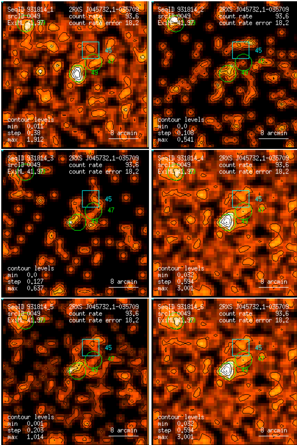
Figure 49: RASS 931814: detection 0049: band rate images, Gaussian filter: (1) PSPC channels 11 – 41, (2) 52 – 90, (3) 91 – 201, (4) 11 – 235, (5) 52 – 201, (6) 11 – 201. Broad band rates in counts/ks. Band rate contour levels in counts/ks/arcmin 2 .
