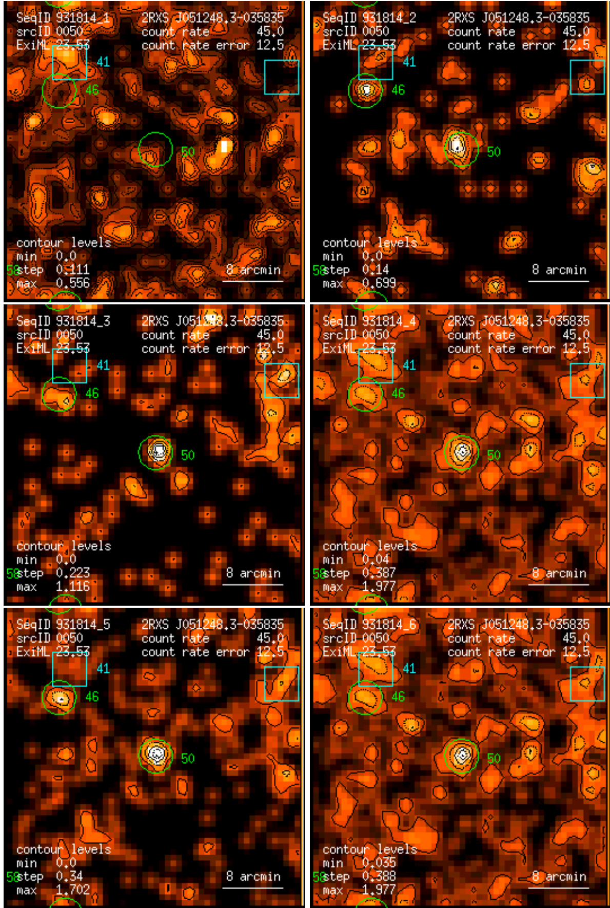
Figure 50: RASS 931814: detection 0050: band rate images, Gaussian filter: (1) PSPC channels 11 – 41, (2) 52 – 90, (3) 91 – 201, (4) 11 – 235, (5) 52 – 201, (6) 11 – 201. Broad band rates in counts/ks. Band rate contour levels in counts/ks/arcmin 2 .
