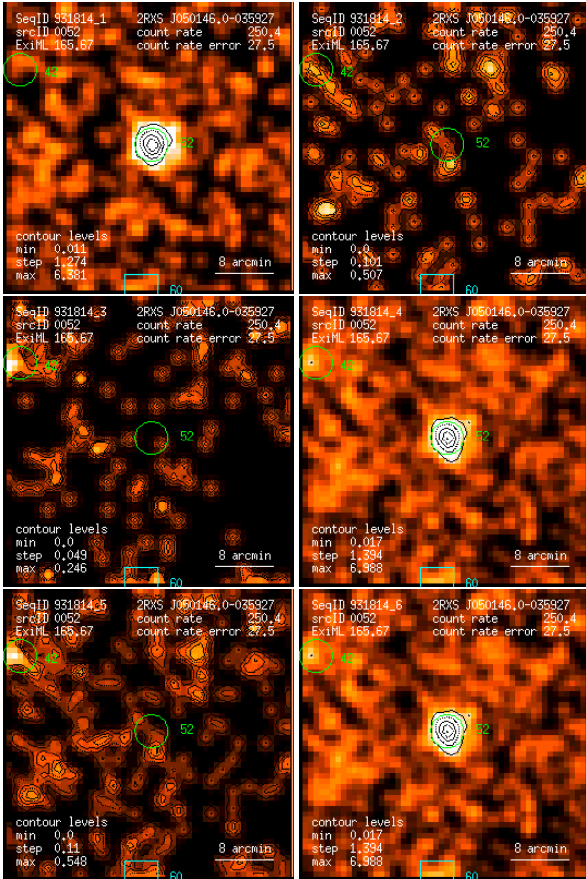
Figure 52: RASS 931814: detection 0052: band rate images, Gaussian filter: (1) PSPC channels 11 – 41, (2) 52 – 90, (3) 91 – 201, (4) 11 – 235, (5) 52 – 201, (6) 11 – 201. Broad band rates in counts/ks. Band rate contour levels in counts/ks/arcmin 2 .
