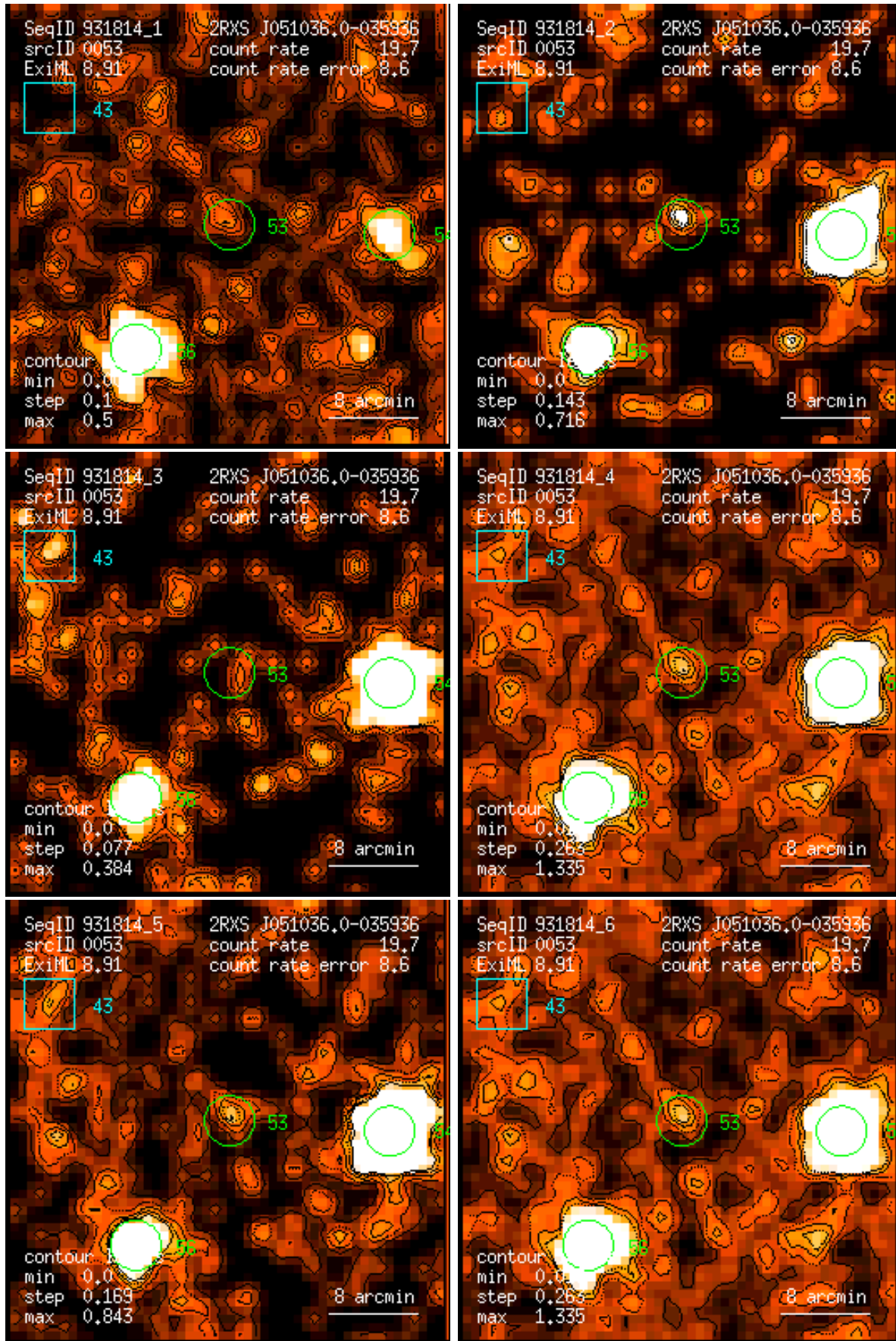
Figure 53: RASS 931814: detection 0053: band rate images, Gaussian filter: (1) PSPC channels 11 – 41, (2) 52 – 90, (3) 91 – 201, (4) 11 – 235, (5) 52 – 201, (6) 11 – 201. Broad band rates in counts/ks. Band rate contour levels in counts/ks/arcmin 2 .
