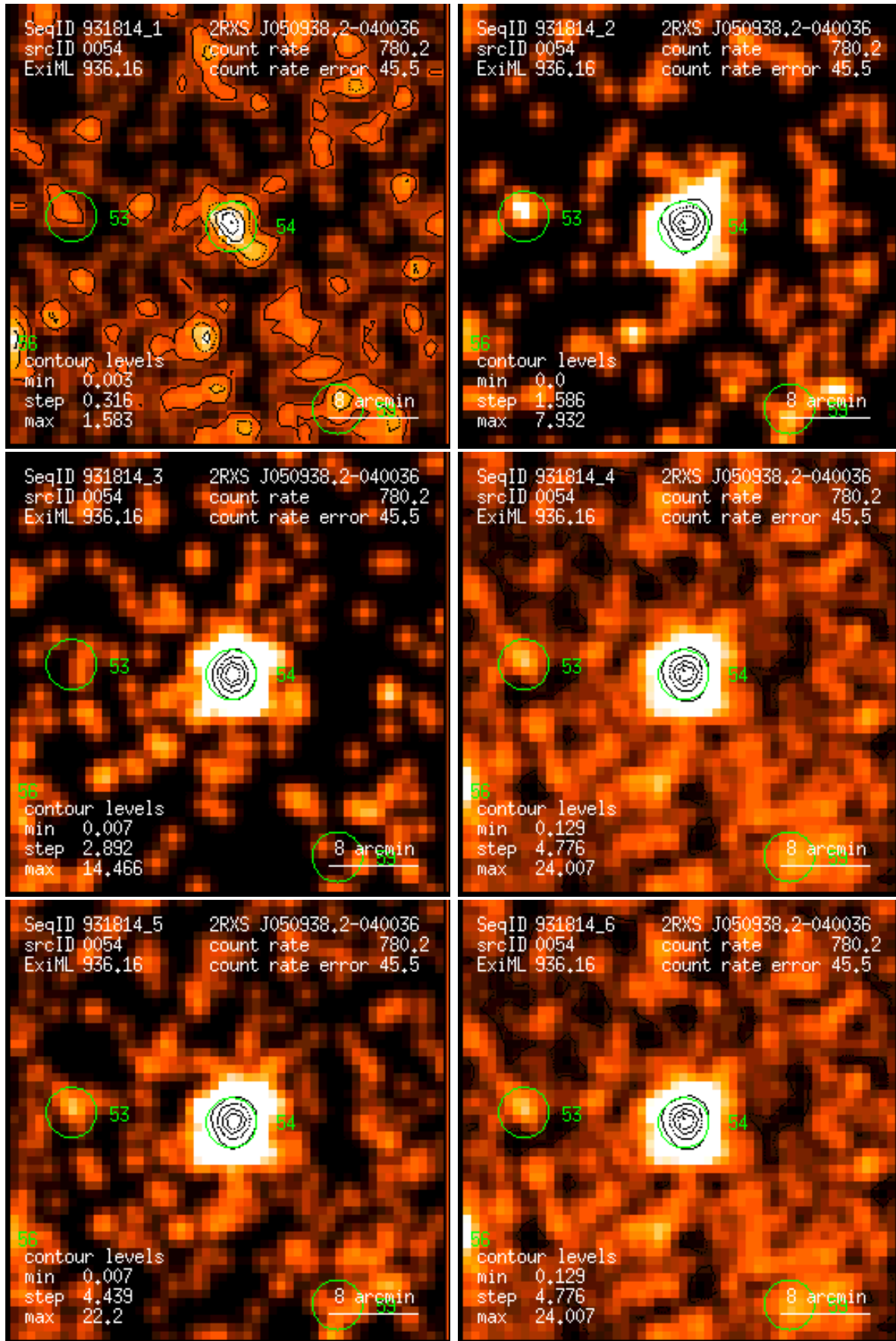
Figure 54: RASS 931814: detection 0054: band rate images, Gaussian filter: (1) PSPC channels 11 – 41, (2) 52 – 90, (3) 91 – 201, (4) 11 – 235, (5) 52 – 201, (6) 11 – 201. Broad band rates in counts/ks. Band rate contour levels in counts/ks/arcmin 2 .
