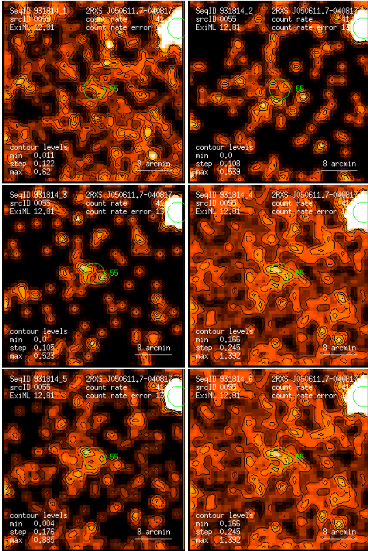
Figure 55: RASS 931814: detection 0055: band rate images, Gaussian filter: (1) PSPC channels 11 – 41, (2) 52 – 90, (3) 91 – 201, (4) 11 – 235, (5) 52 – 201, (6) 11 – 201. Broad band rates in counts/ks. Band rate contour levels in counts/ks/arcmin 2 .
