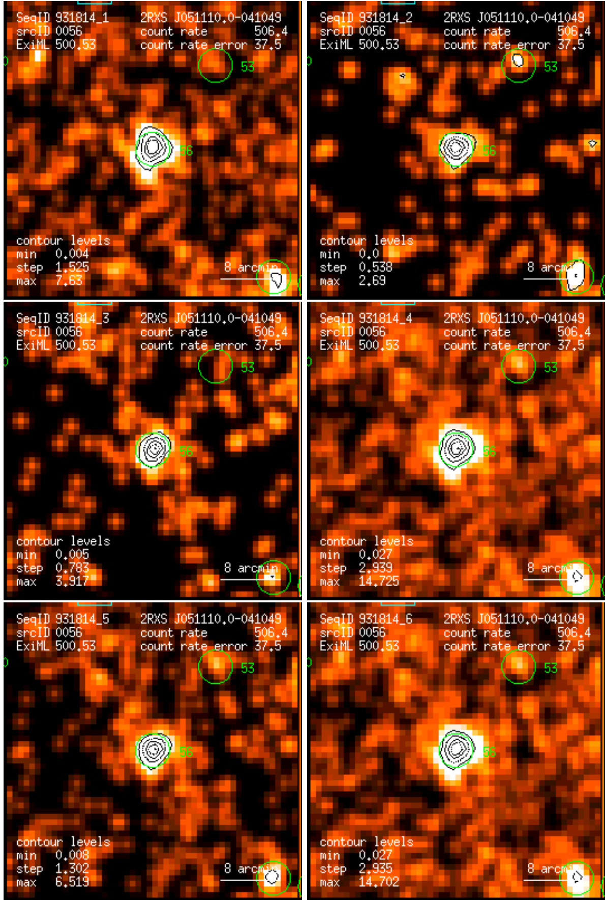
Figure 56: RASS 931814: detection 0056: band rate images, Gaussian filter: (1) PSPC channels 11 – 41, (2) 52 – 90, (3) 91 – 201, (4) 11 – 235, (5) 52 – 201, (6) 11 – 201. Broad band rates in counts/ks. Band rate contour levels in counts/ks/arcmin 2 .
