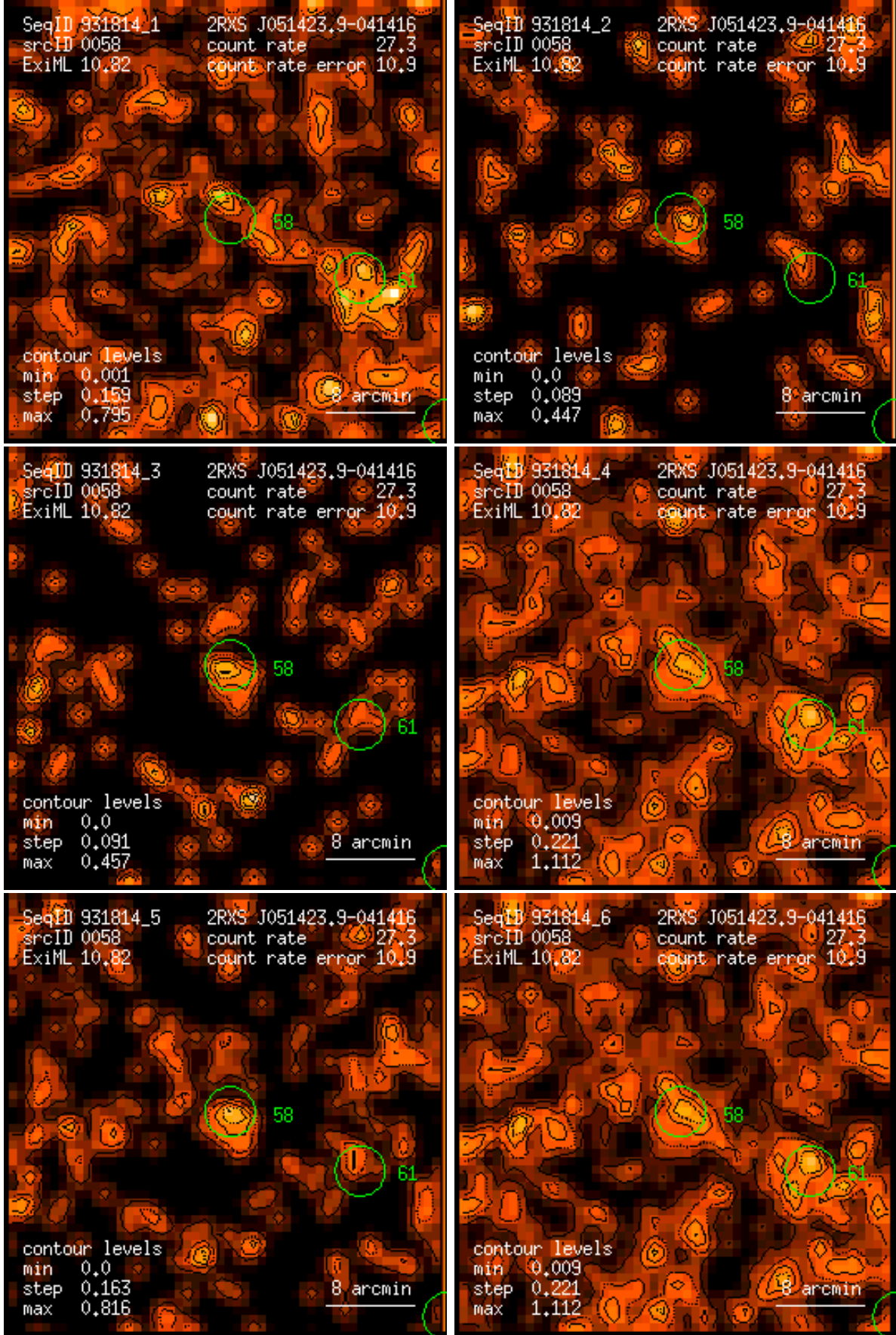
Figure 58: RASS 931814: detection 0058: band rate images, Gaussian filter: (1) PSPC channels 11 – 41, (2) 52 – 90, (3) 91 – 201, (4) 11 – 235, (5) 52 – 201, (6) 11 – 201. Broad band rates in counts/ks. Band rate contour levels in counts/ks/arcmin 2 .
