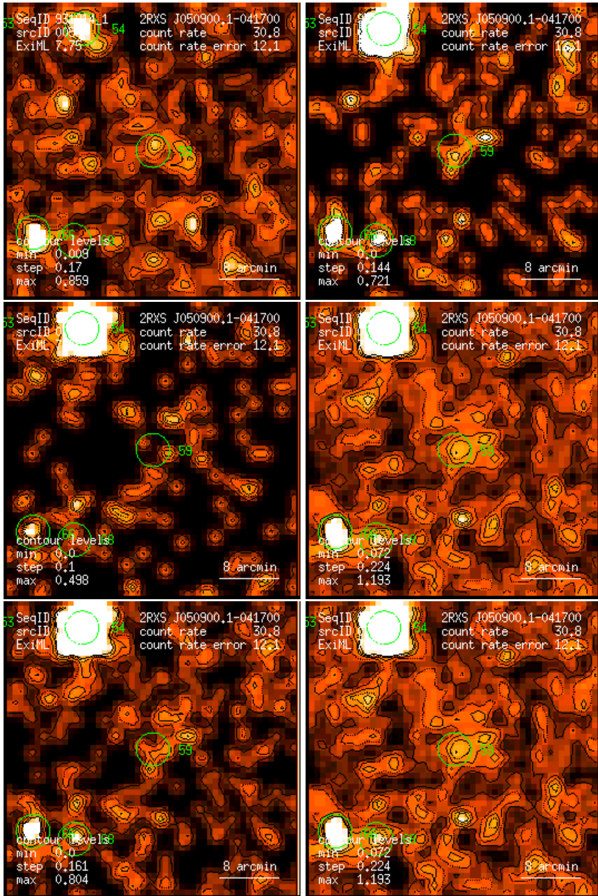
Figure 59: RASS 931814: detection 0059: band rate images, Gaussian filter: (1) PSPC channels 11 – 41, (2) 52 – 90, (3) 91 – 201, (4) 11 – 235, (5) 52 – 201, (6) 11 – 201. Broad band rates in counts/ks. Band rate contour levels in counts/ks/arcmin 2 .
