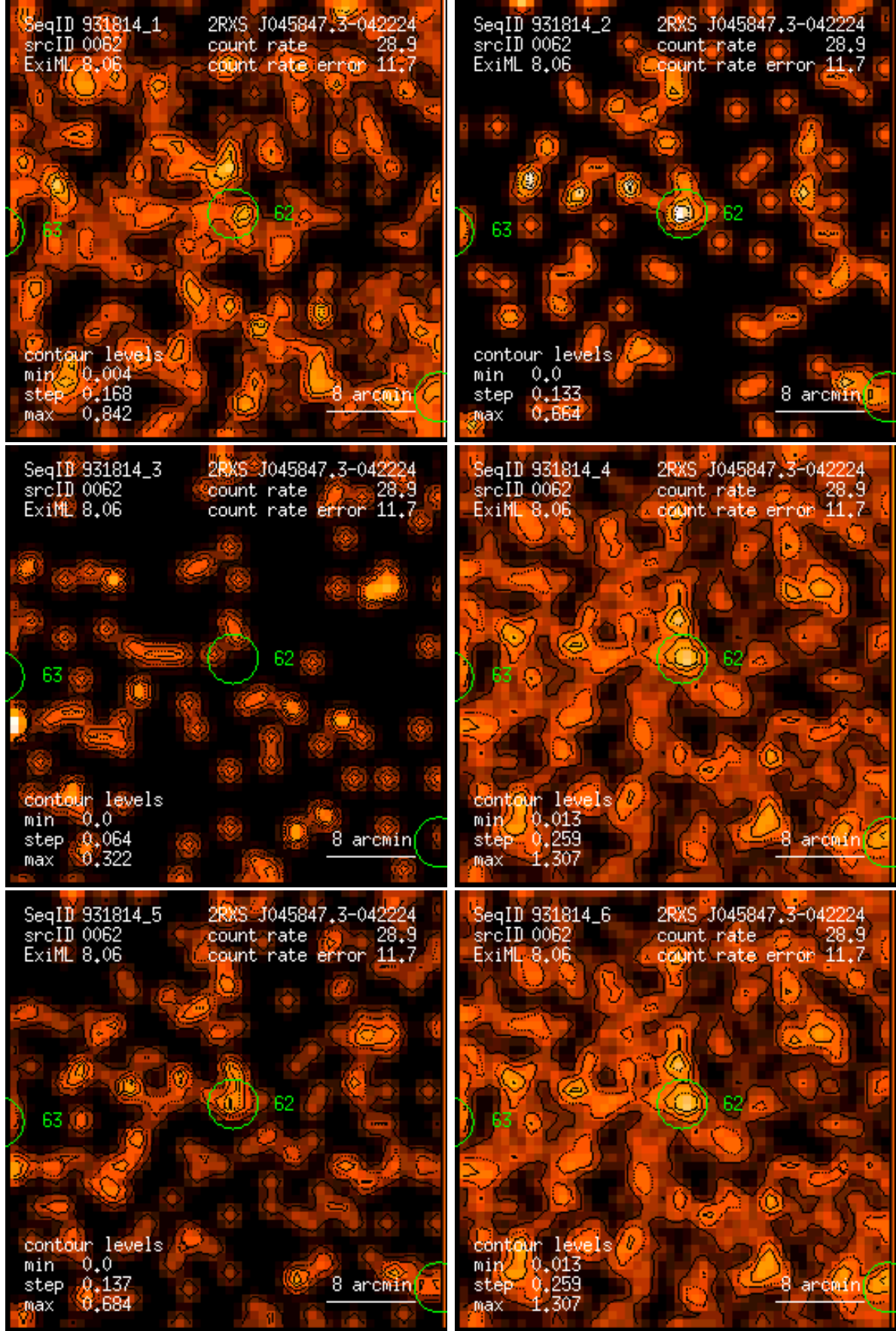
Figure 62: RASS 931814: detection 0062: band rate images, Gaussian filter: (1) PSPC channels 11 – 41, (2) 52 – 90, (3) 91 – 201, (4) 11 – 235, (5) 52 – 201, (6) 11 – 201. Broad band rates in counts/ks. Band rate contour levels in counts/ks/arcmin 2 .
