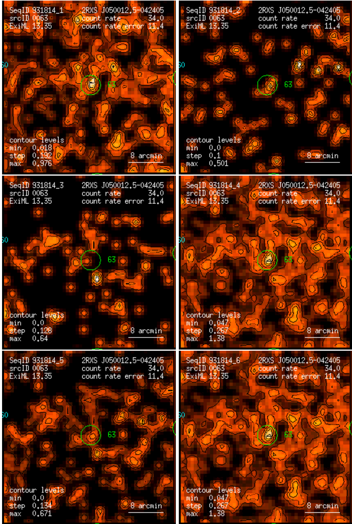
Figure 63: RASS 931814: detection 0063: band rate images, Gaussian filter: (1) PSPC channels 11 – 41, (2) 52 – 90, (3) 91 – 201, (4) 11 – 235, (5) 52 – 201, (6) 11 – 201. Broad band rates in counts/ks. Band rate contour levels in counts/ks/arcmin 2 .
